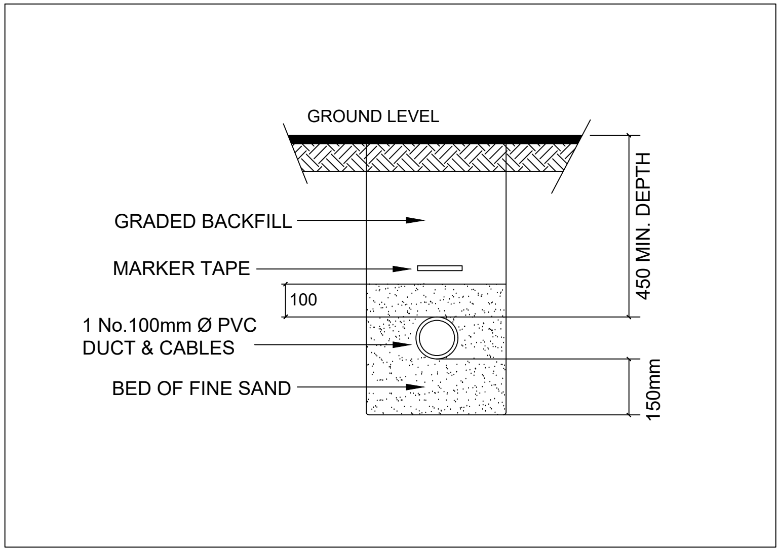
DETAIL D - TYPICAL TRENCH DETAIL
