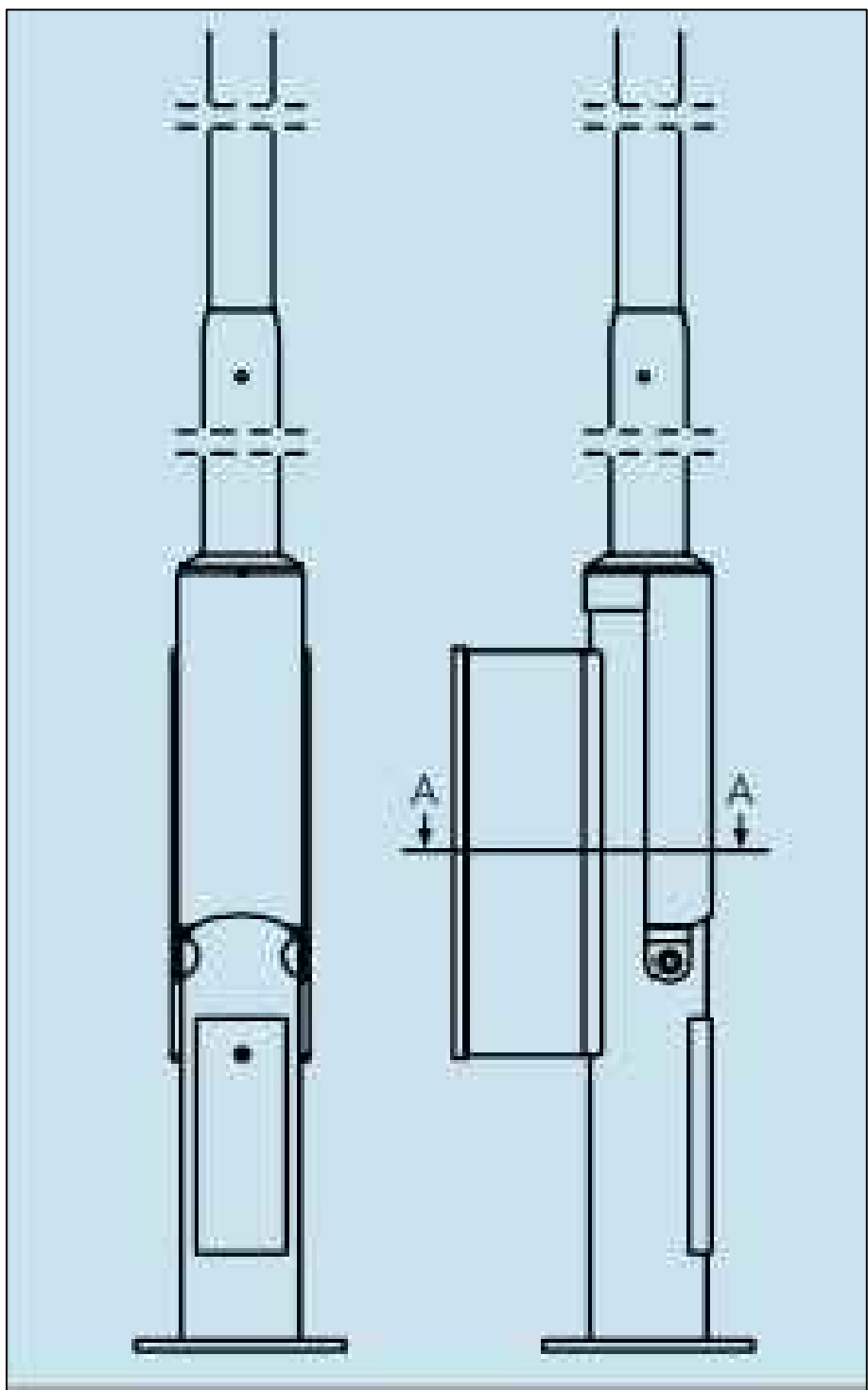
DETAIL B - HINGED SPORTS COLUMN
