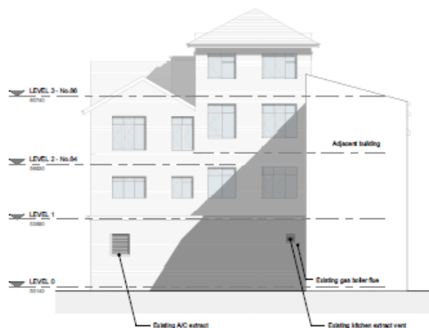
3. Rear - Existing 1:100
