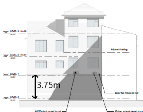
1. Rear - Proposed 1:100
