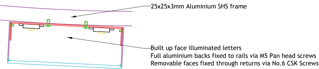
Detail B 1:4 @ A3
