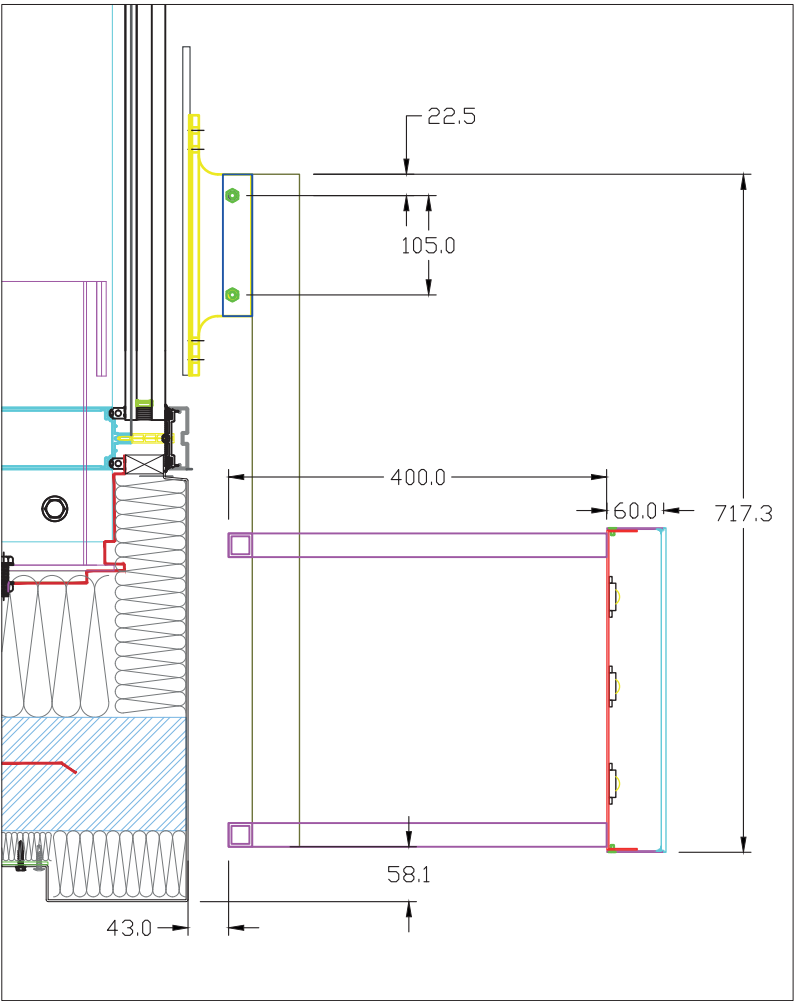
Side view (1:8 @ A3)
