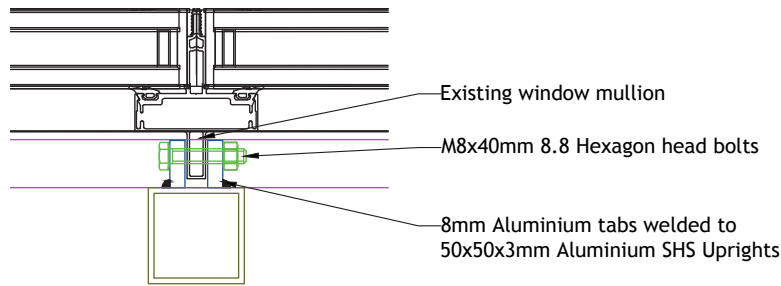
Detail A 1:4 @ A3
