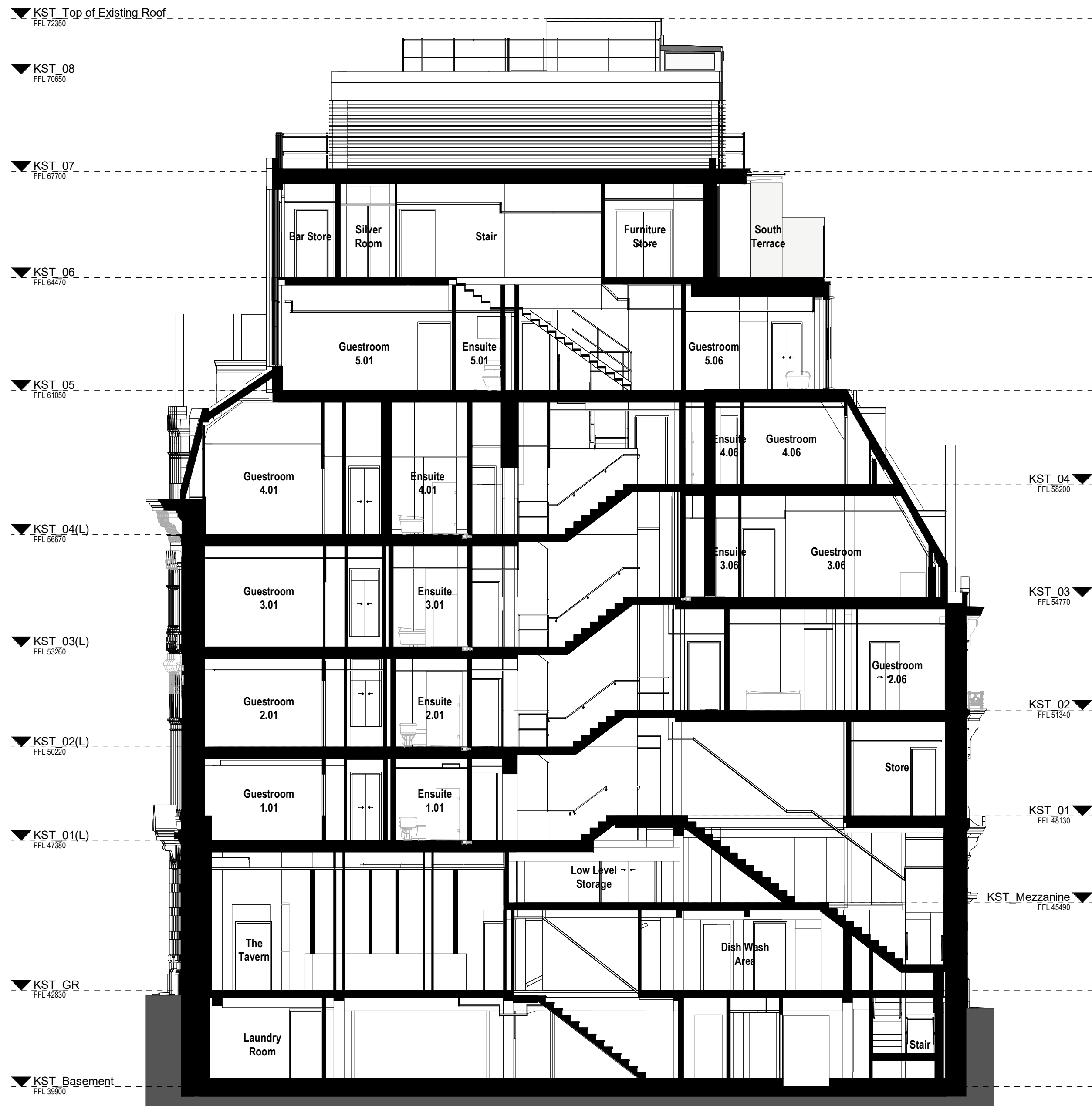
A Existing Section AA 1:100
