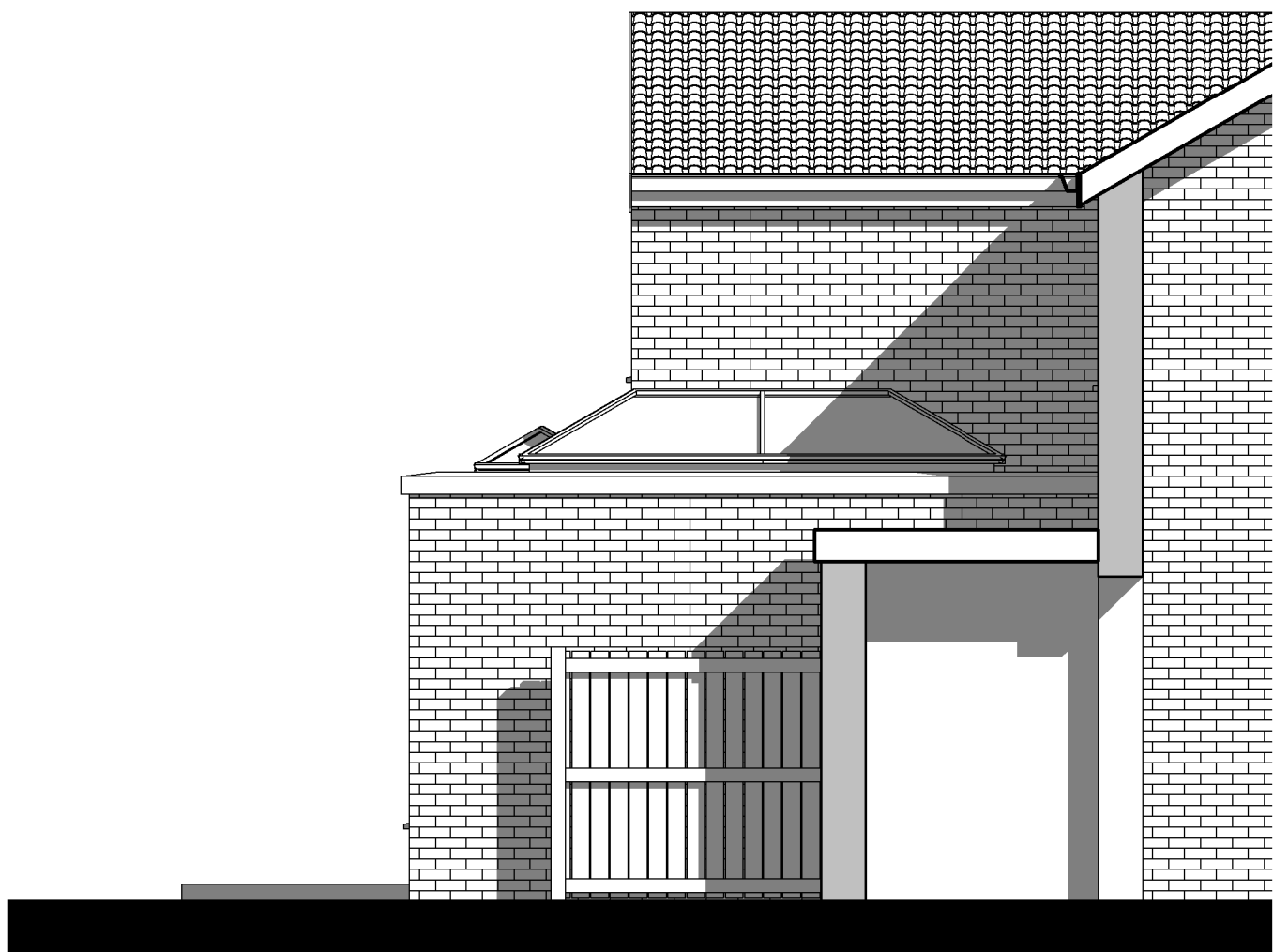
Proposed Side Elevation1 1 : 50
