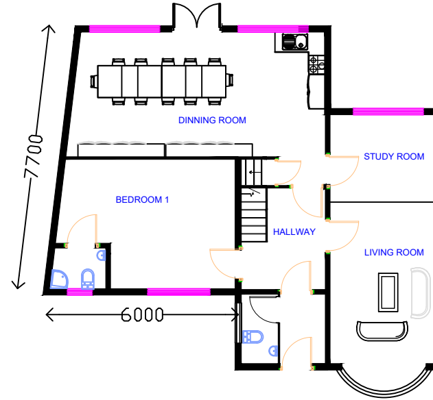
3 Proposed Ground Floor Plan 1 : 50
