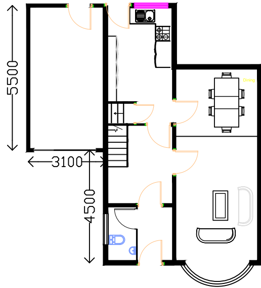
1 Existing Ground Floor Plan 1 : 50
