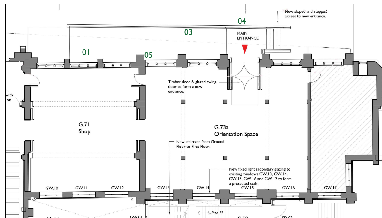
3 Proposed Plan 901 1:200
