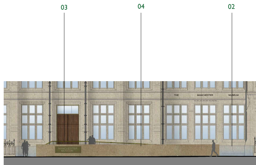
2 901 Approved Elevation 1:200
