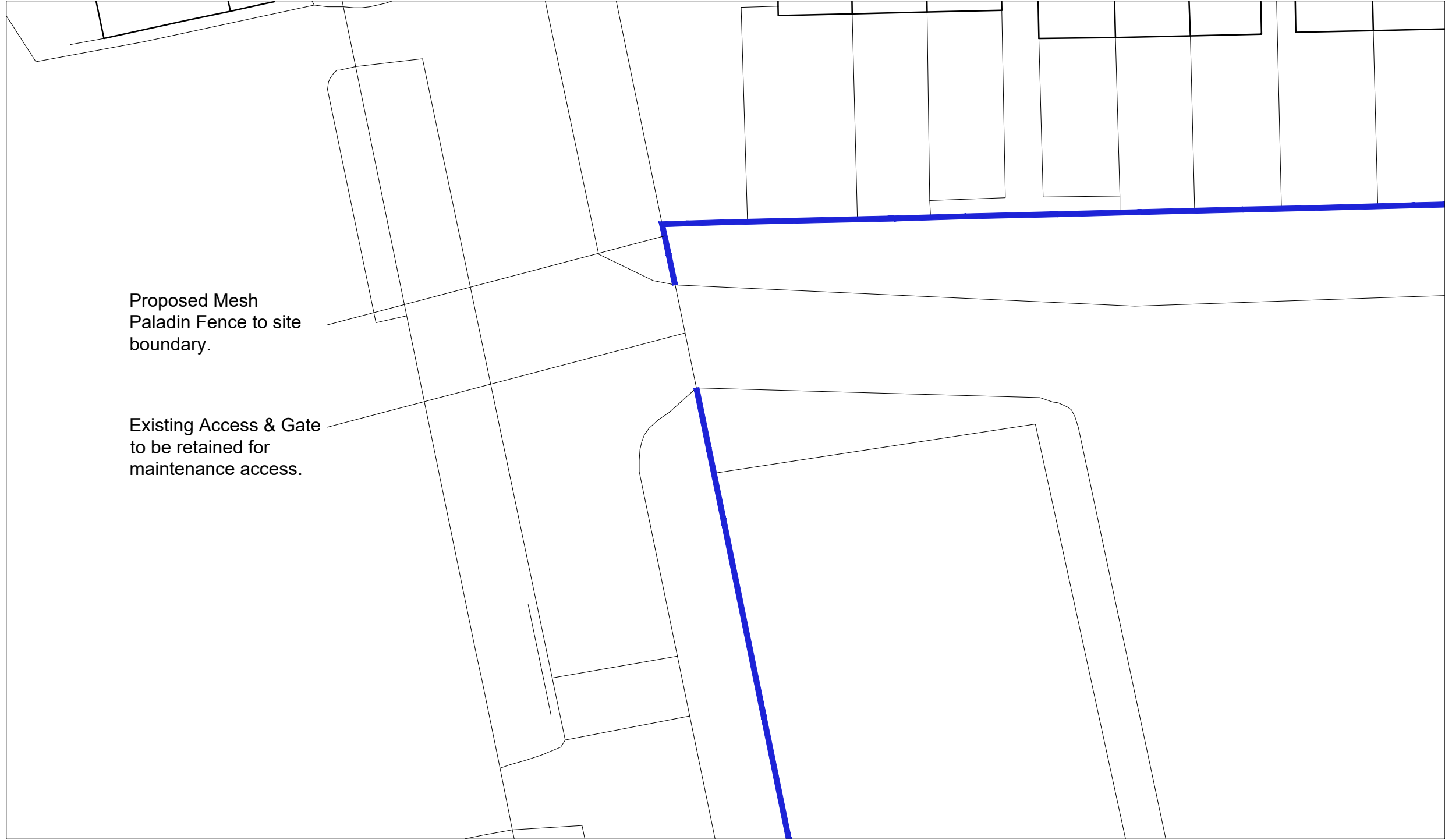
Maintenance Access Position, Scale 1:250
