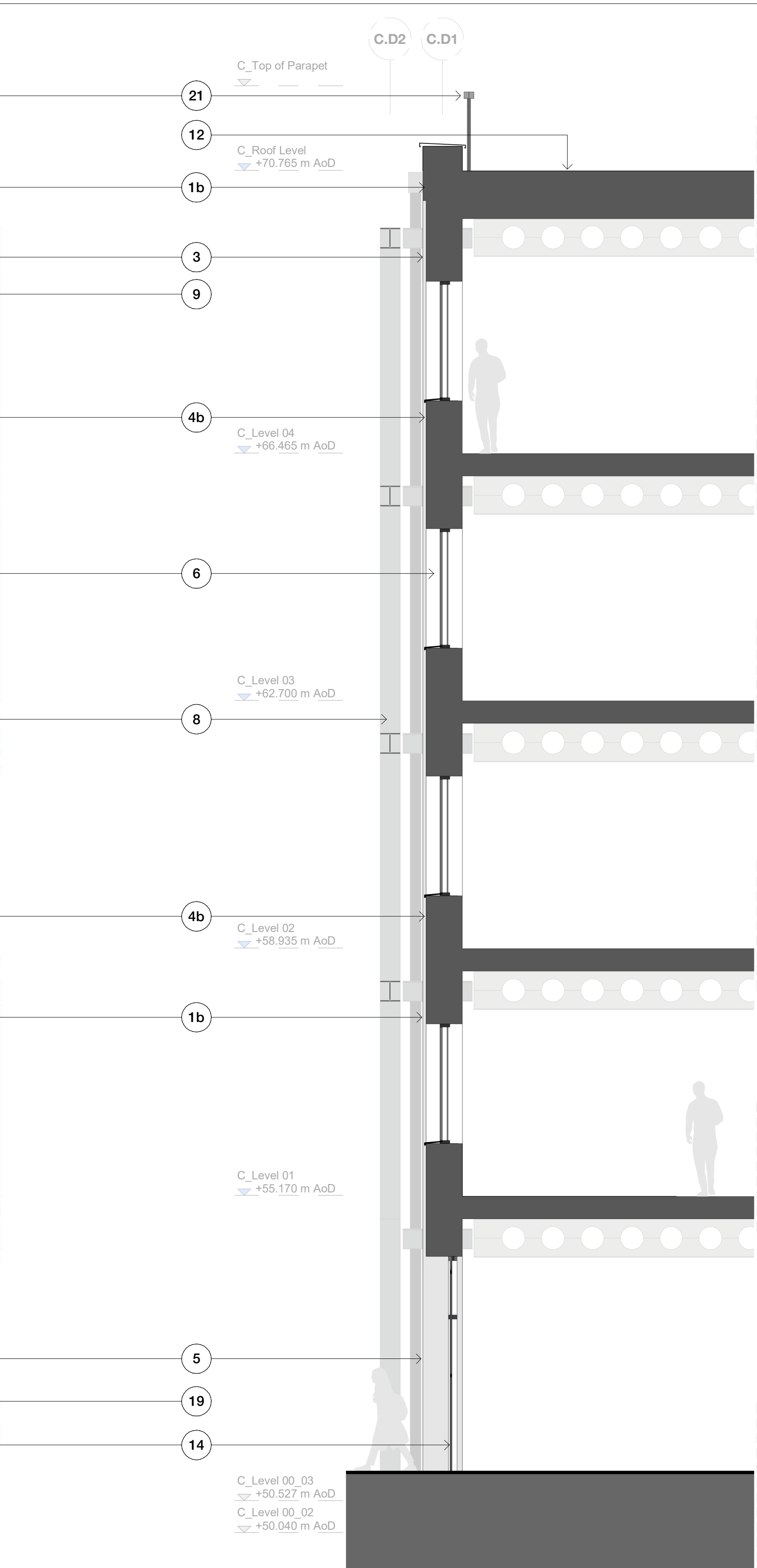
Building C - Section B-B 1 : 50
