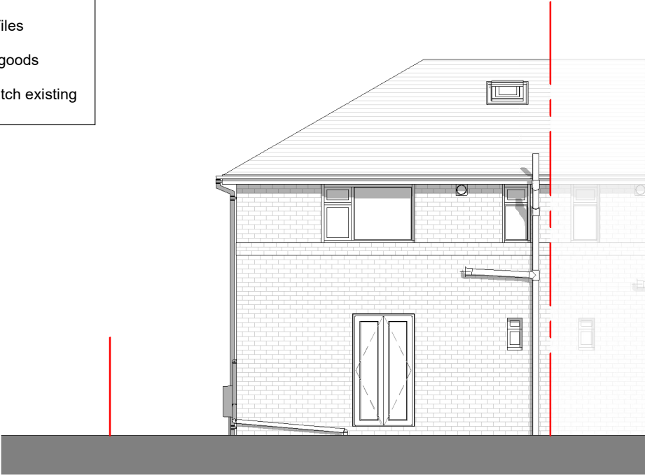
Rear Elevation 1 : 100
