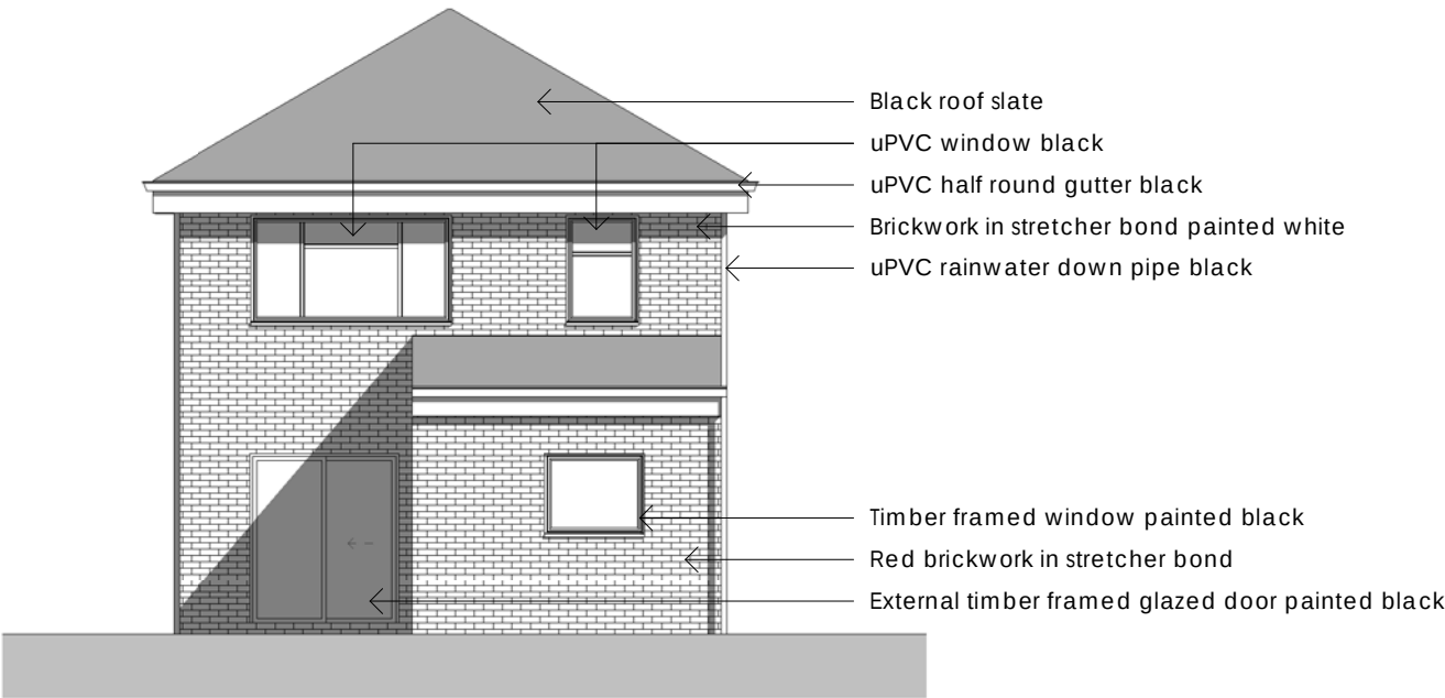
4 West Elevation- Existing 1 : 100
