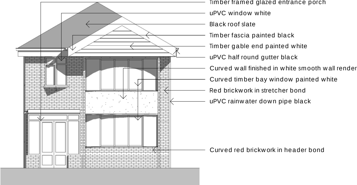
4 West Elevation- Existing 1 : 100
