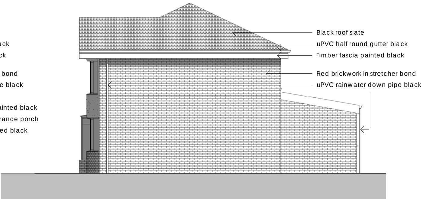
2 South Elevation- Existing 1 : 100
