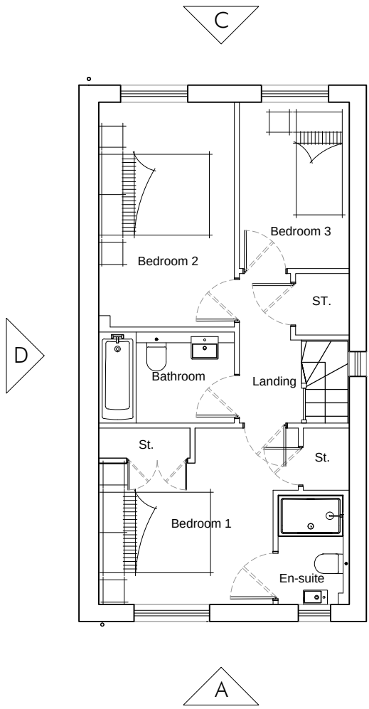
First Floor 43 Sq.m/468 Sq.ft
