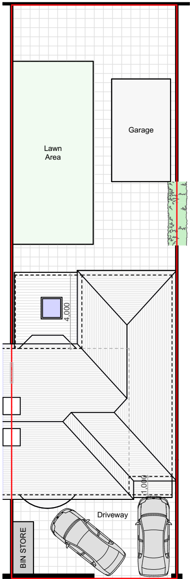
PROPOSED GA SITE PLAN @1:200
