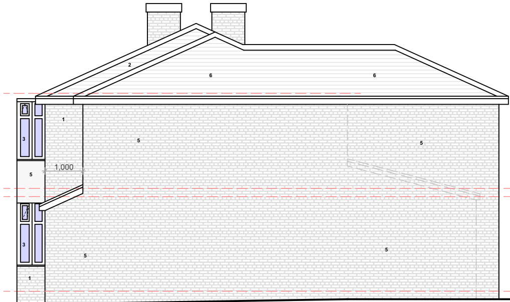
PROPOSED GA SIDE ELEVATION 1 @1:100
