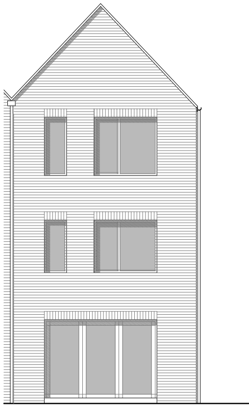
C - Rear Elevation
