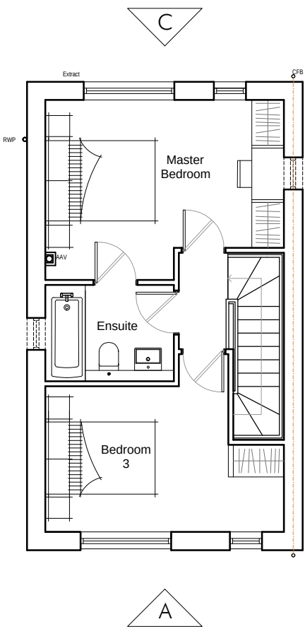
Second Floor 36m 2 /388ft 2
