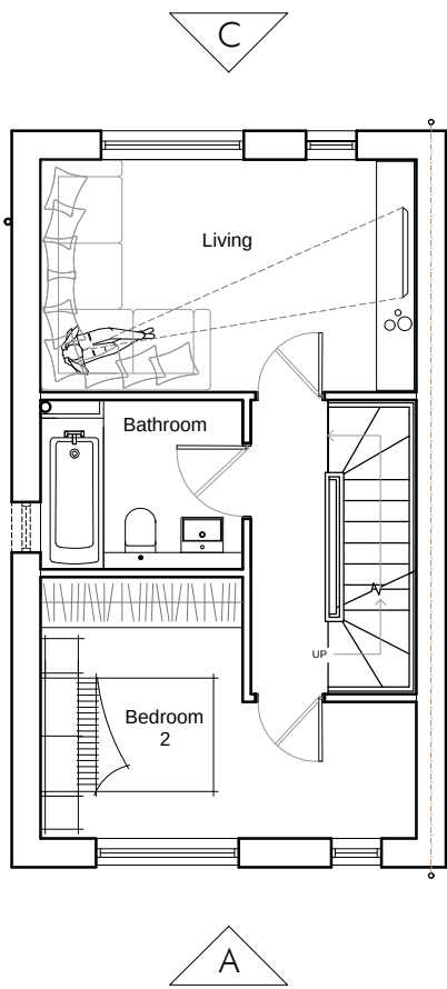
First Floor 36m 2 /388ft 2
