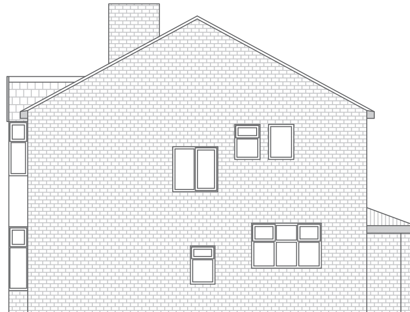
Existing Right hand side Elevation
