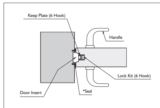
Sliding Panels to One Side
