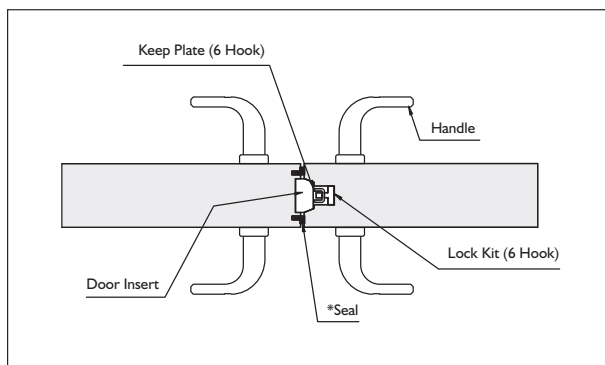
Central Meeting Panels
