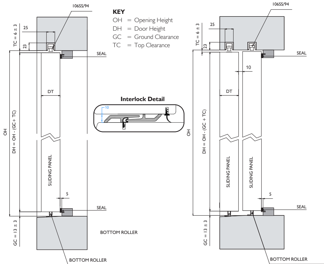
One Fixed and One Sliding Panel Central Meeting Panels
