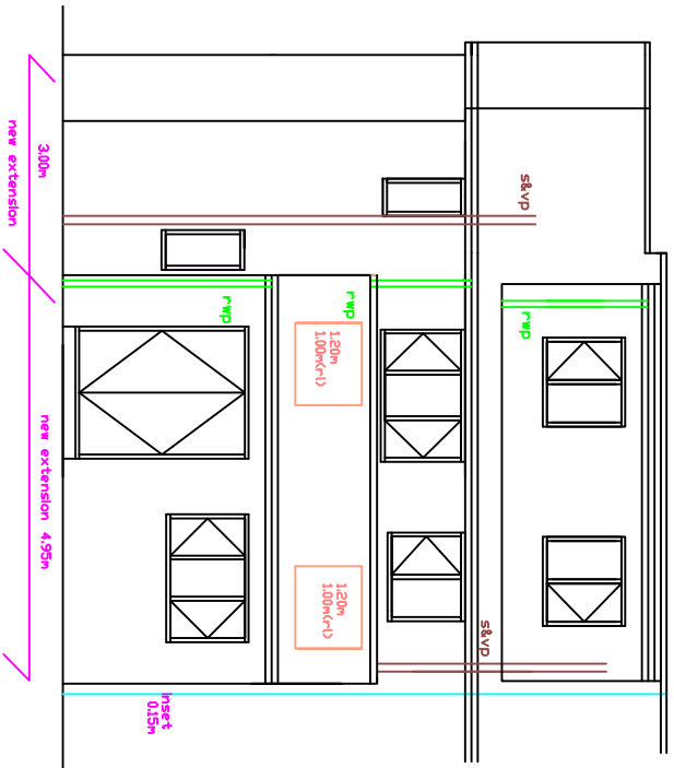
PROPOSED REAR VIEW 1:100
