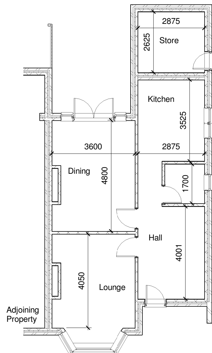
01 Existing Ground Floor Plan 1 : 100
