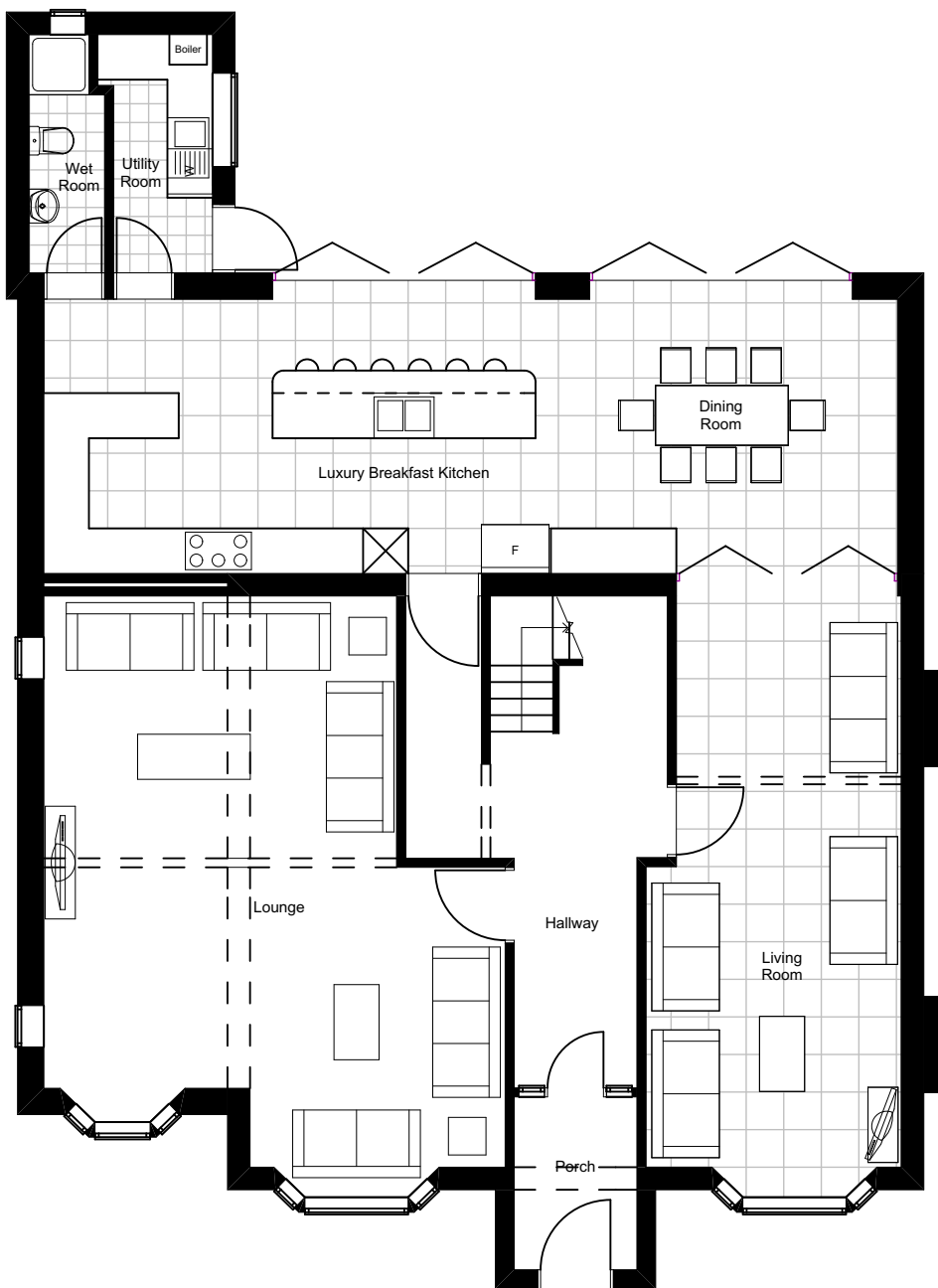
PROPOSED GA GROUND FLOOR PLAN
