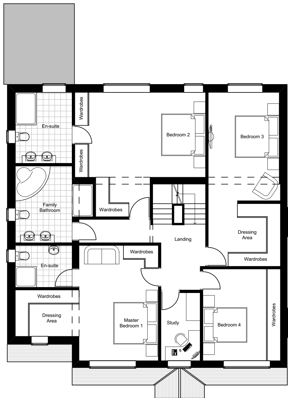
PROPOSED GA SECOND FLOOR PLAN
