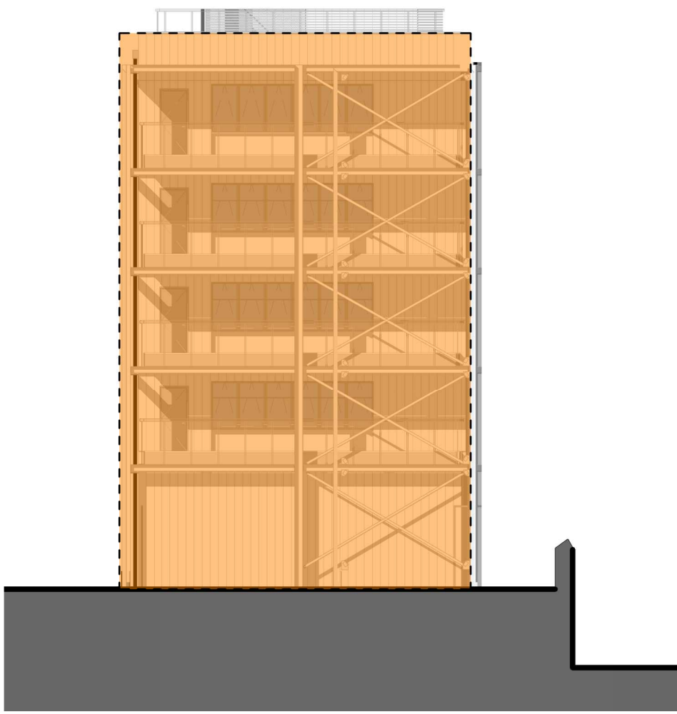
Building B - West Elevation. 1 : 200
