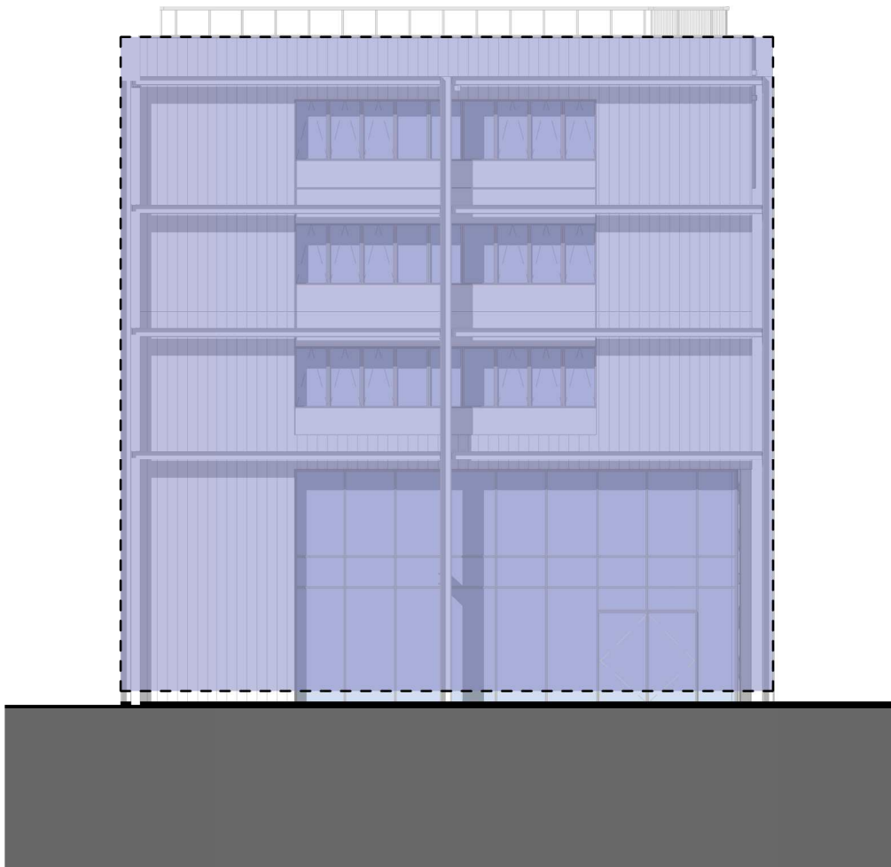
Building B - East Elevation. 1 : 200
