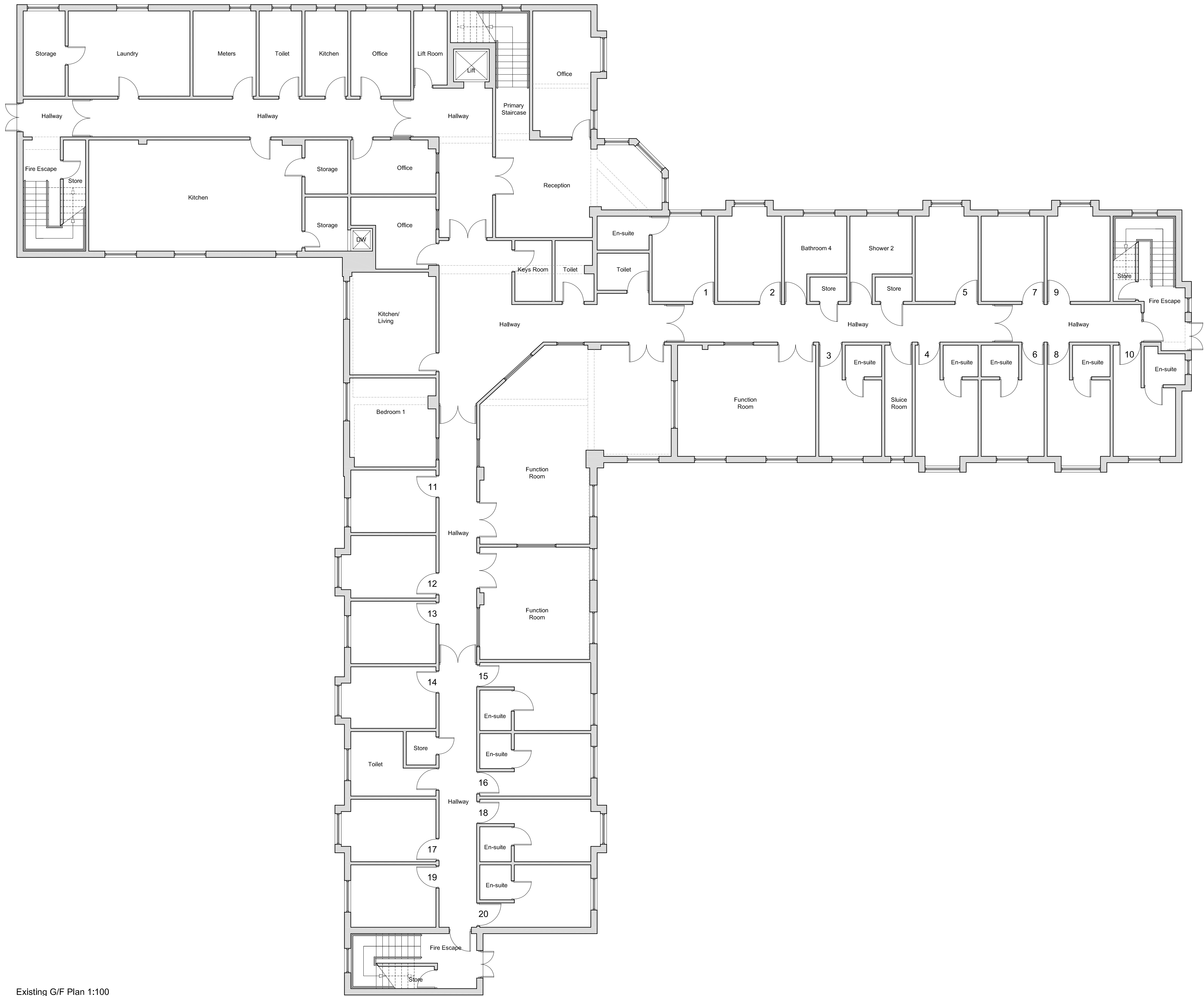
Existing G/F Plan 1:100 Scale Bar 1:100 0 5 10m
