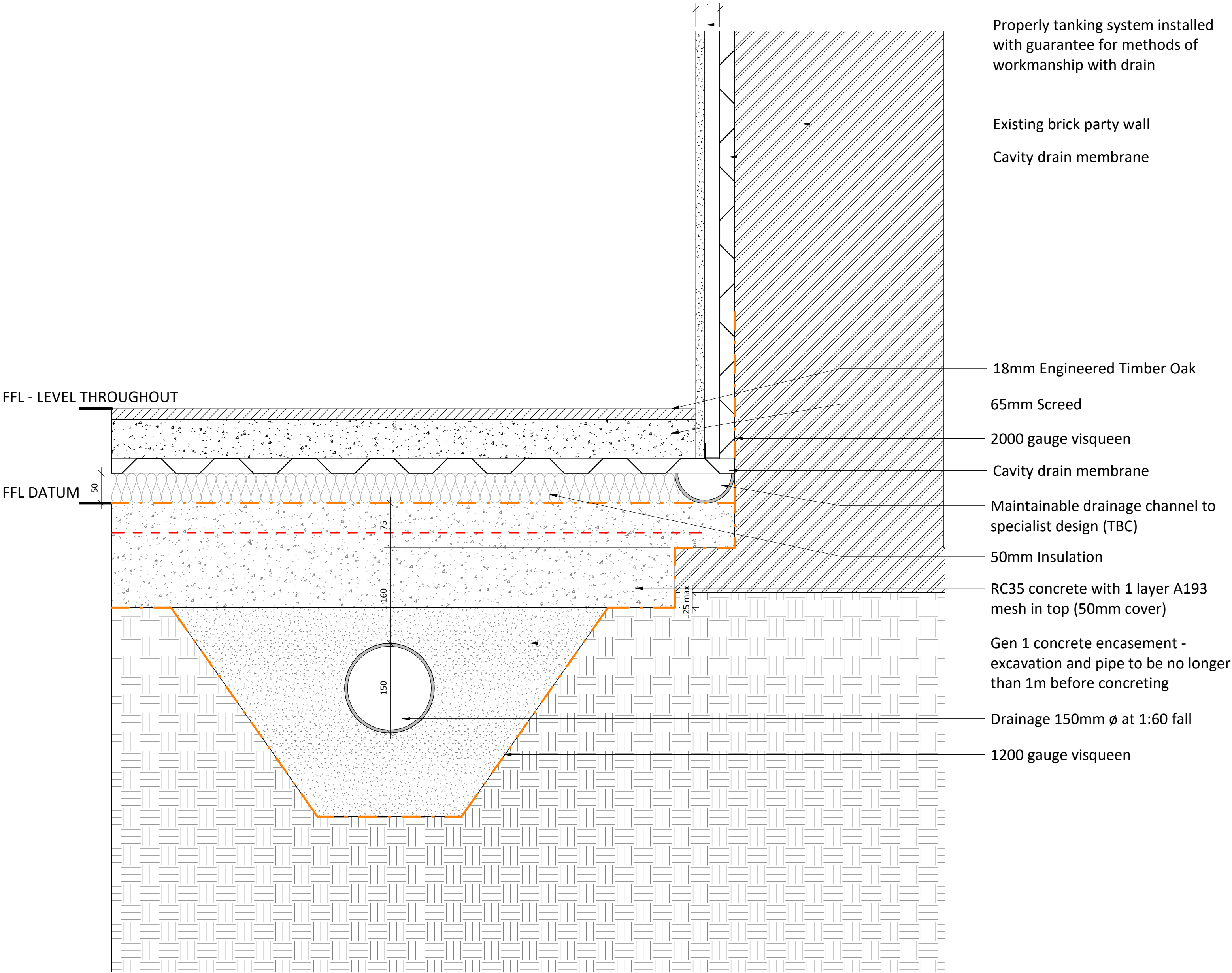
Footings Section 1 : 5
