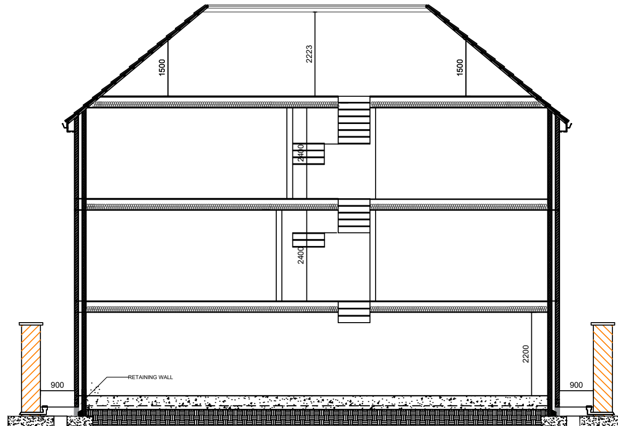
SECTION CC
