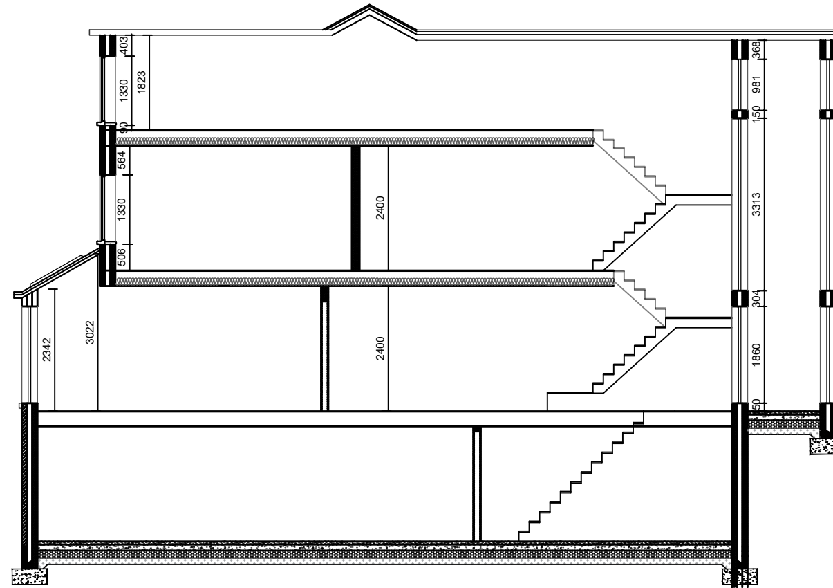
SECTION BB
