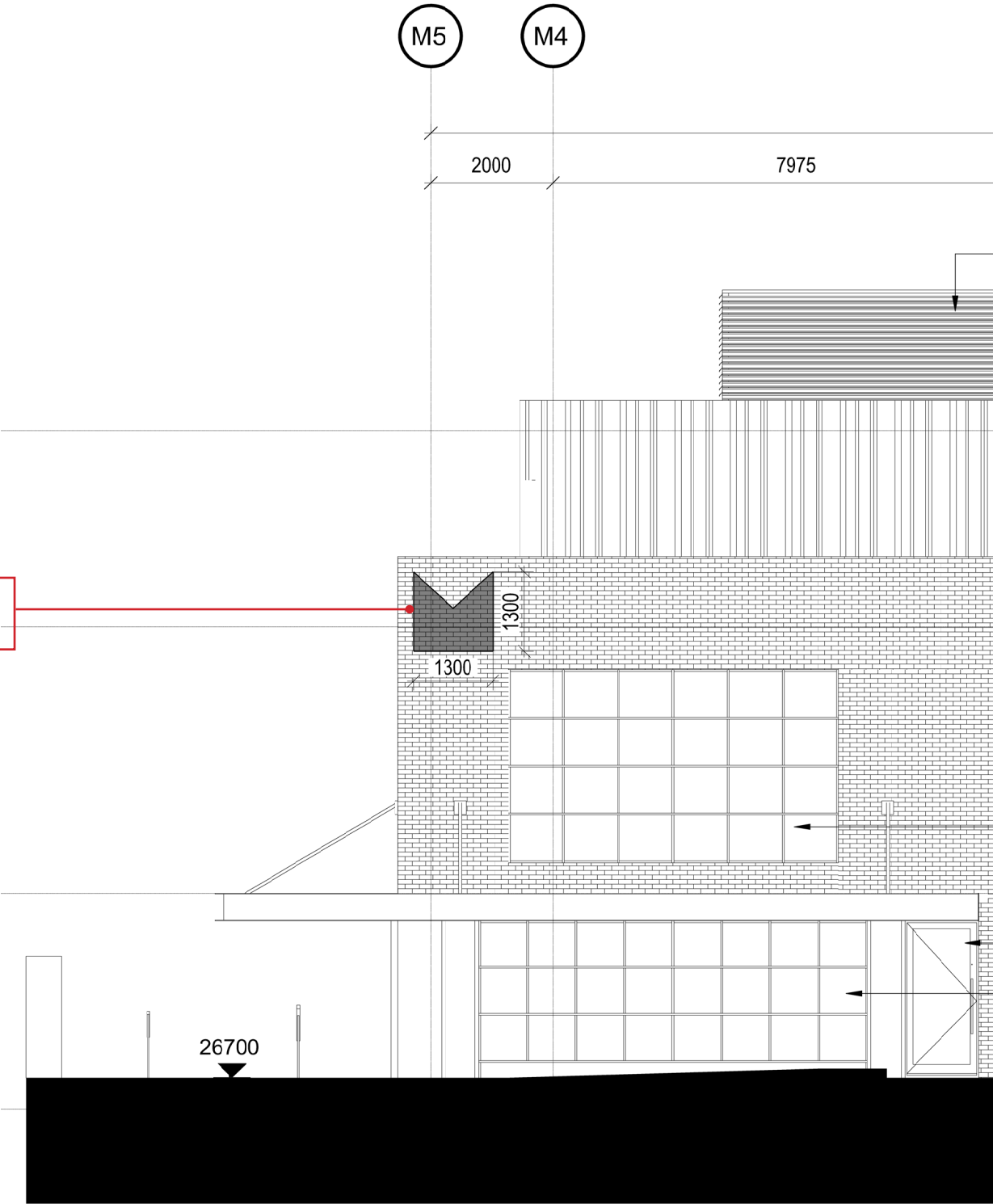
WEST ELEVATION
