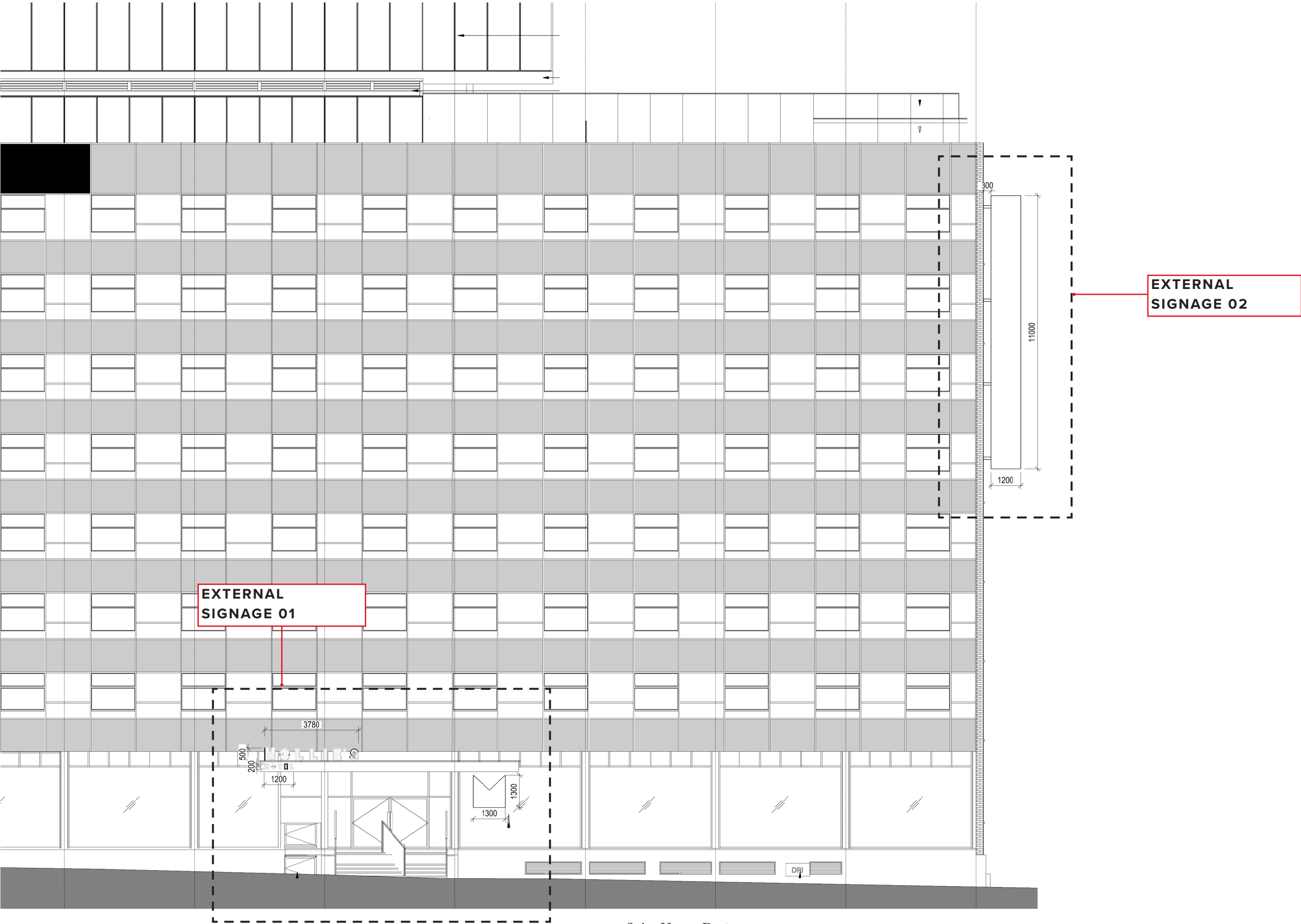
EAST ELEVATION
