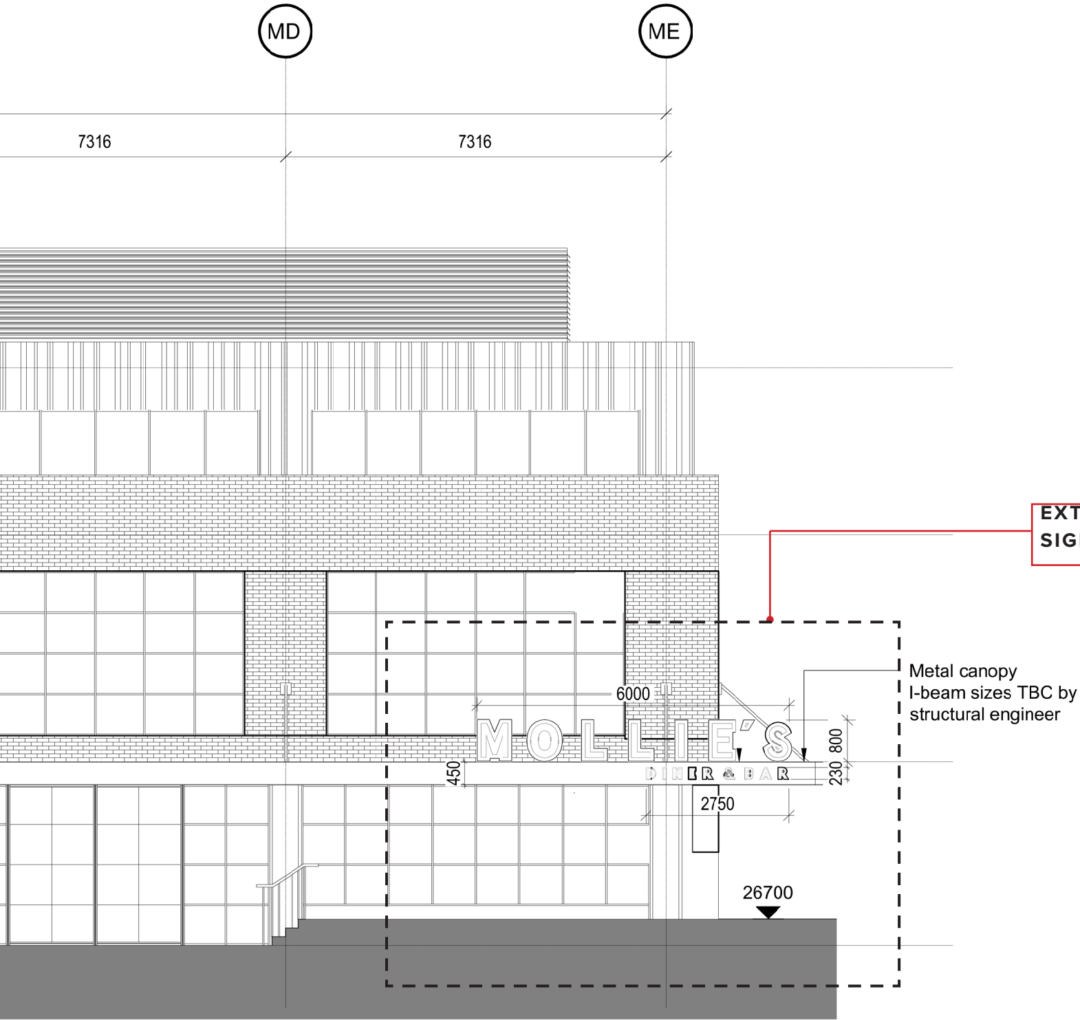
NORTH ELEVATION
