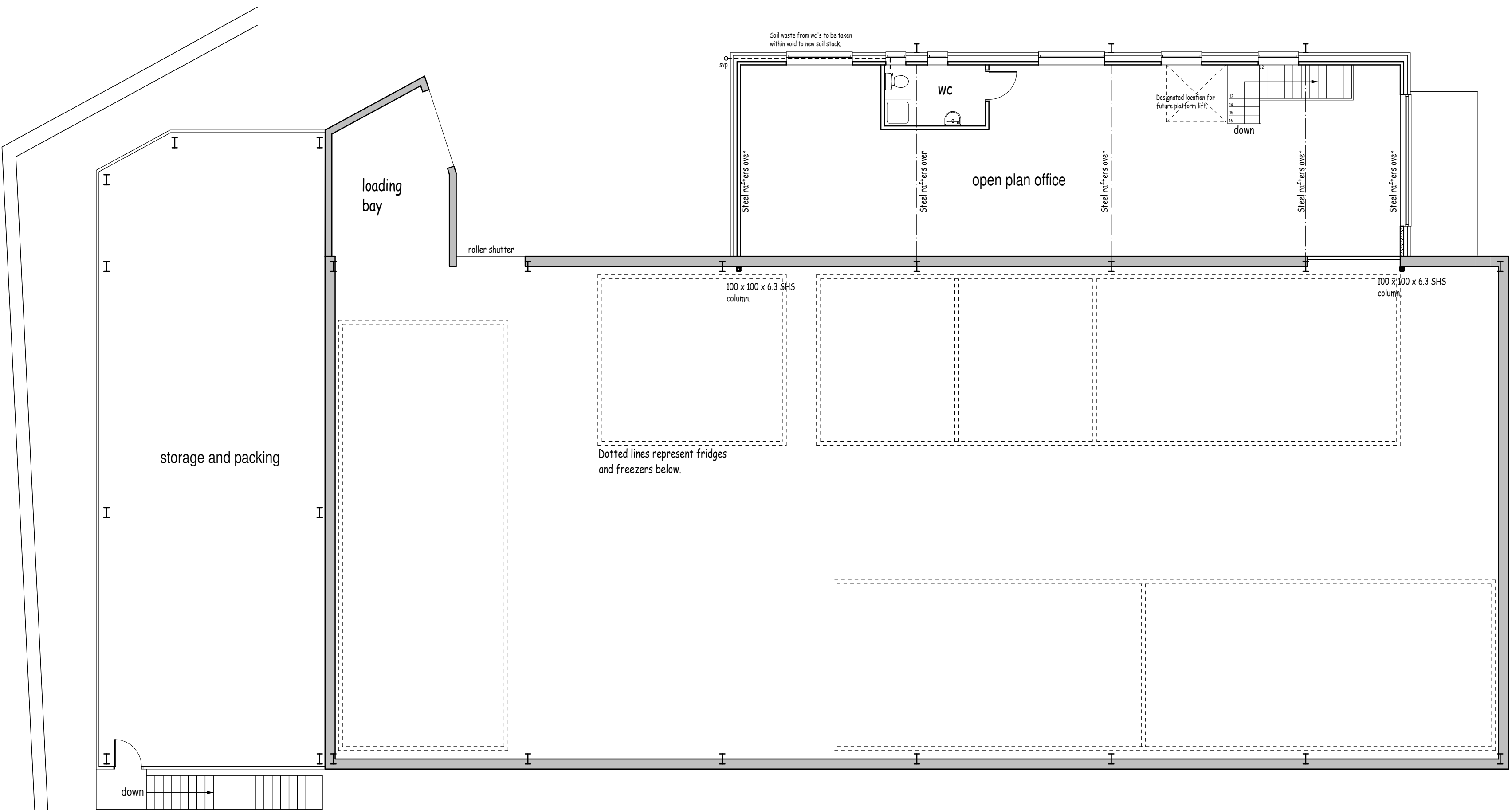
Proposed first floor layout (1:100)
