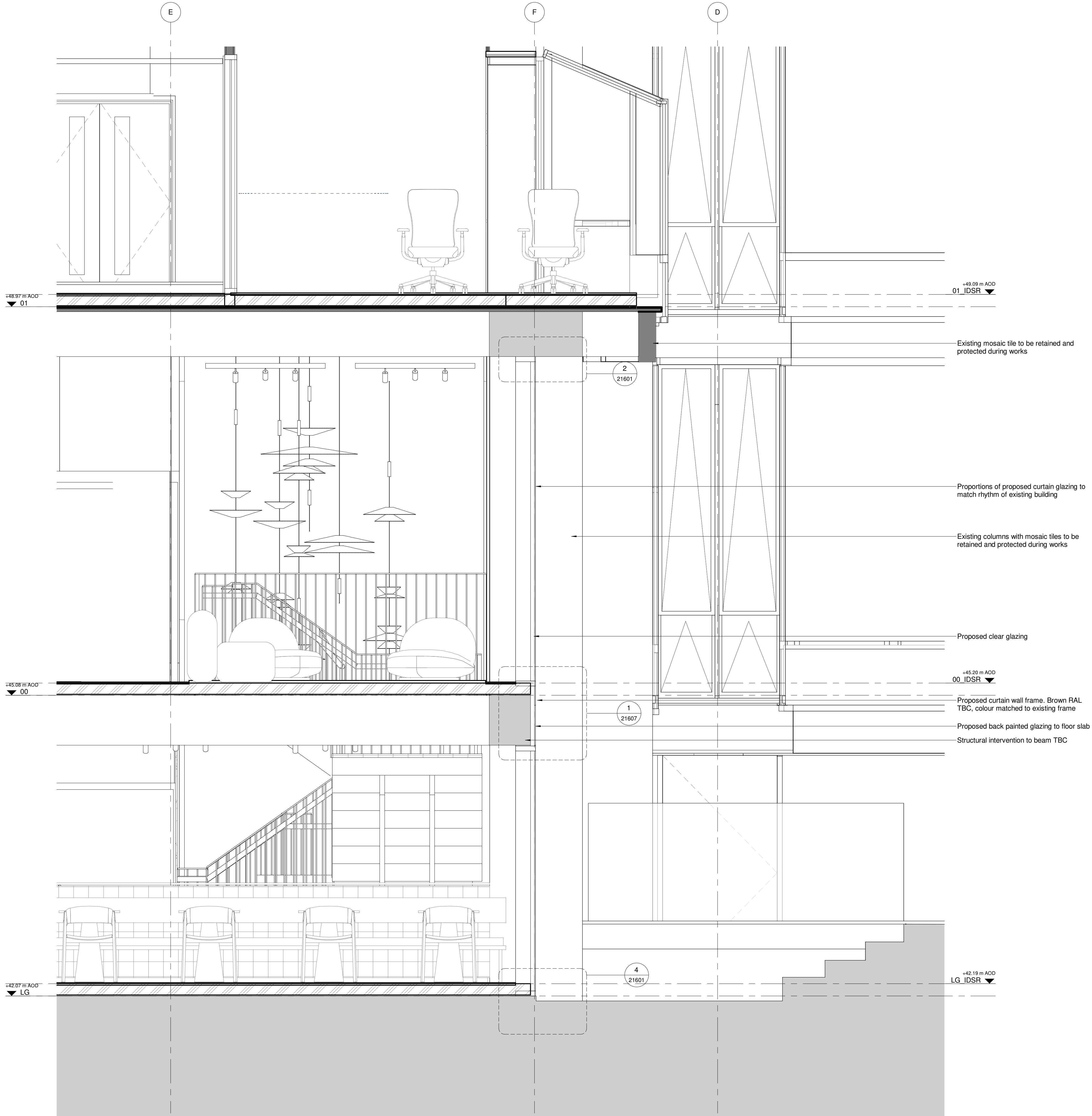
1 Piazza Facade Bay Study Section 21603 1 : 20
