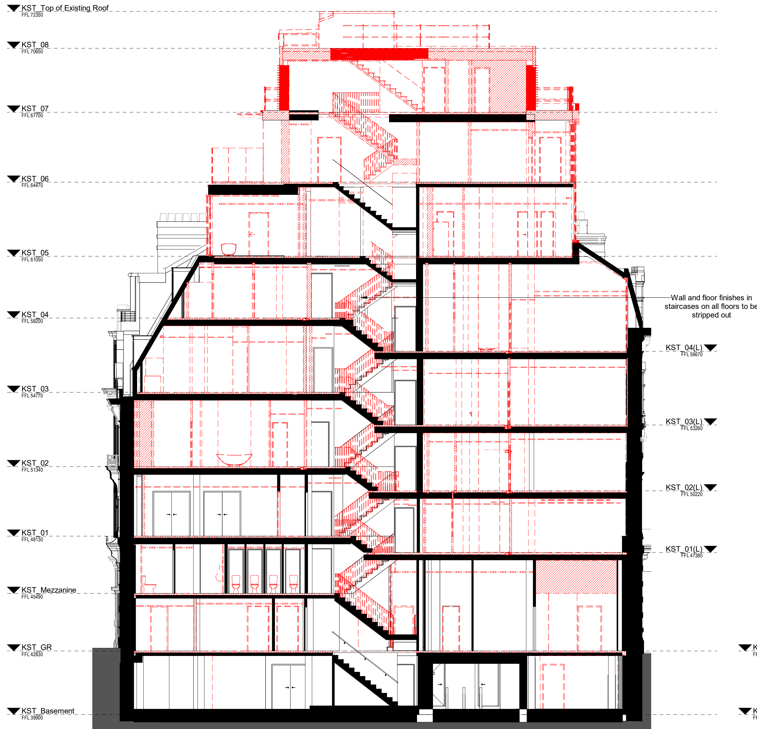
1 Demolition Section CC 1:100
