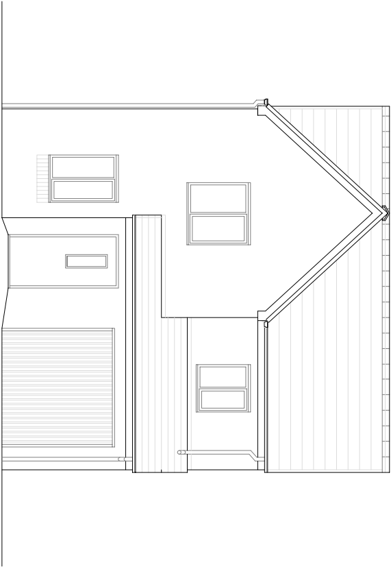
FRONT ELEVATION (EXISTING)
