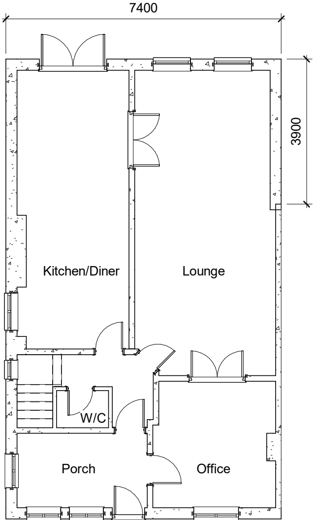
2 Level 0 - Proposed 1 : 100
