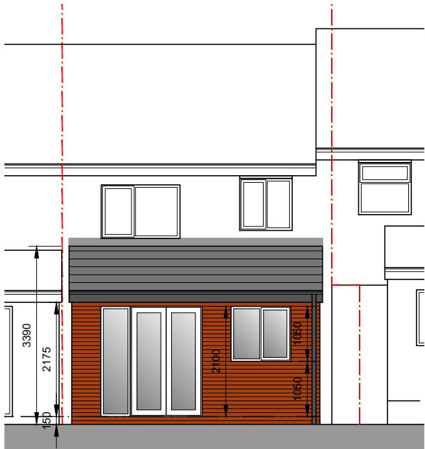
North East Facing Rear Elevation
