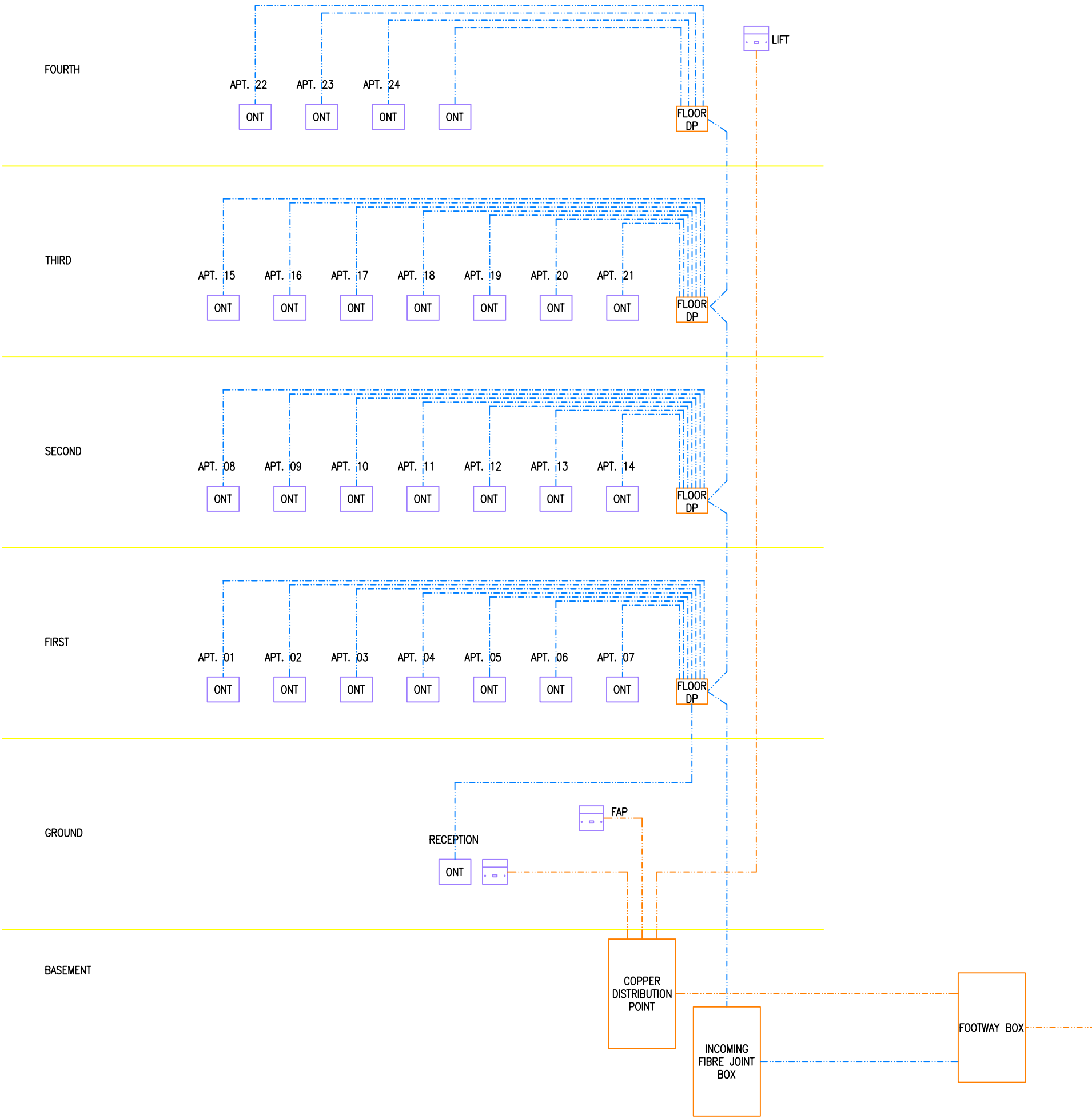
TELECOM DISTRIBUTION SCHEMATIC.(NTS)
