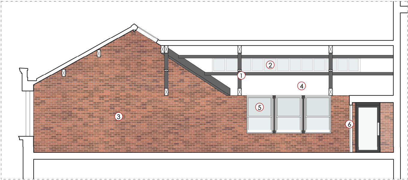
FOURWAYS HOUSE, FIFTH FLOOR PROPOSED SECTION CC' 1.100 @ A3
