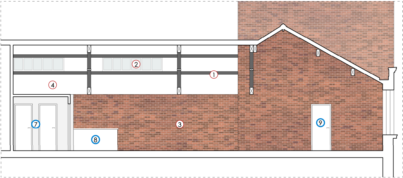
FOURWAYS HOUSE, FIFTH FLOOR PROPOSED SECTION DD' 1.100 @ A3
