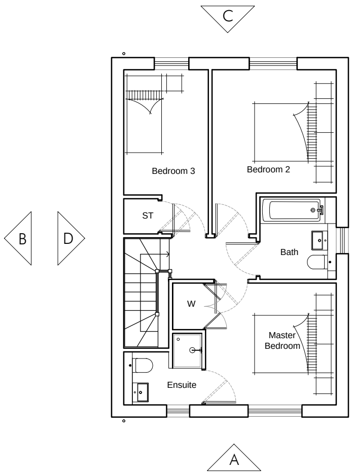
First Floor 48 m²/522ft²
