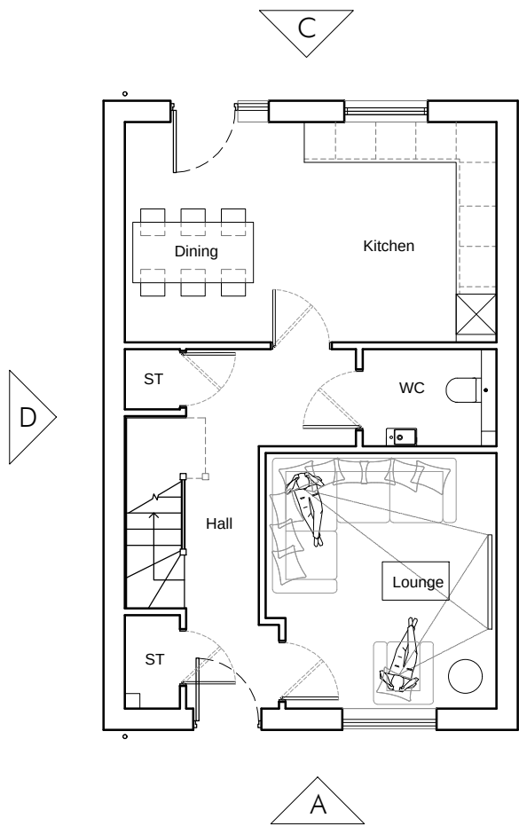
Ground Floor 48 m²/522ft²
