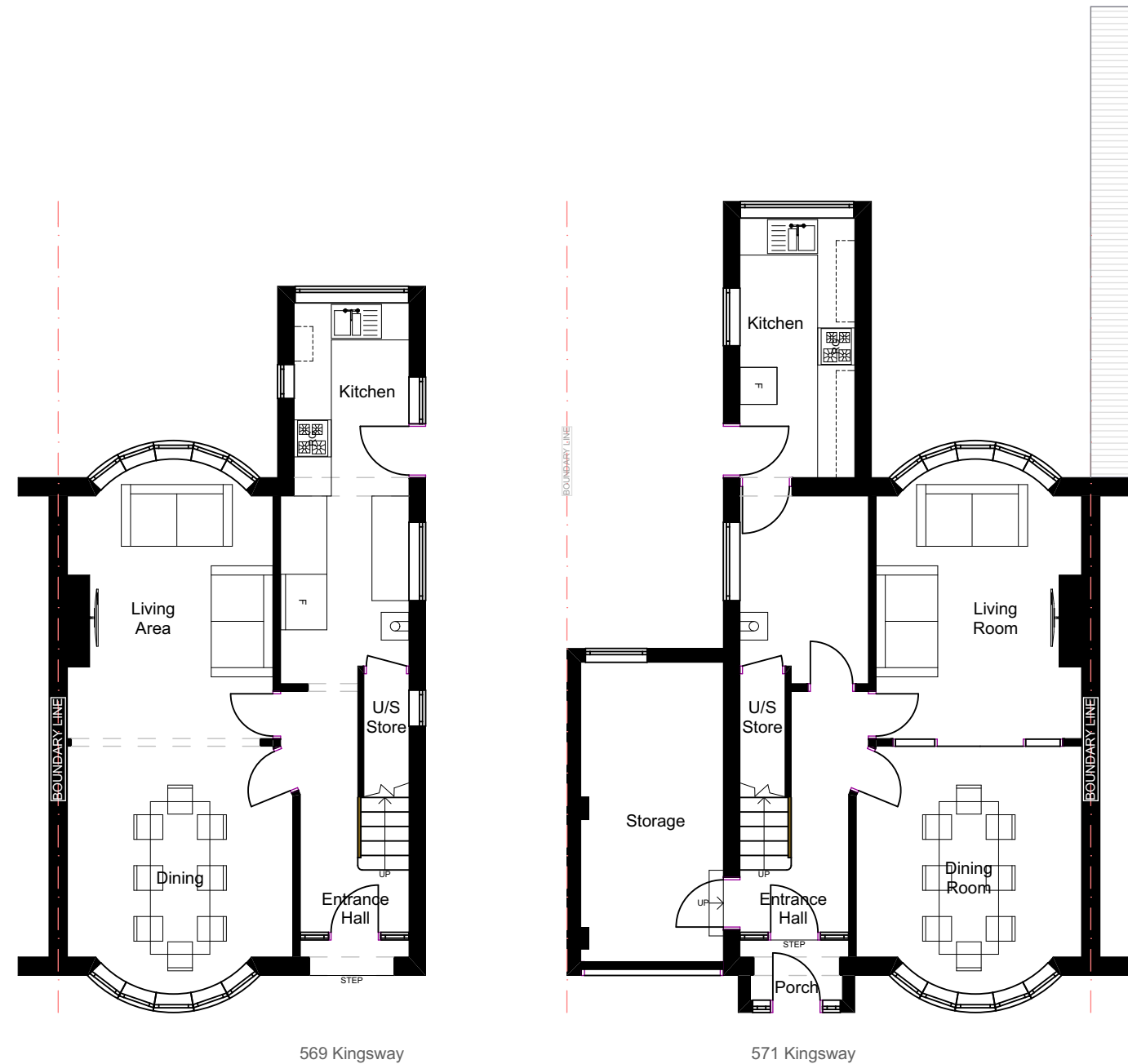
EXISTING GA GROUND FLOOR PLANS
