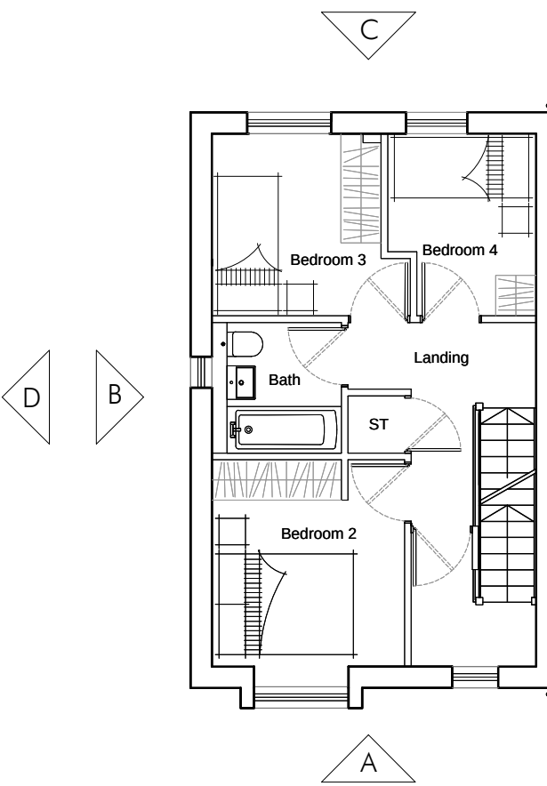
First Floor 39 m²/416ft²
