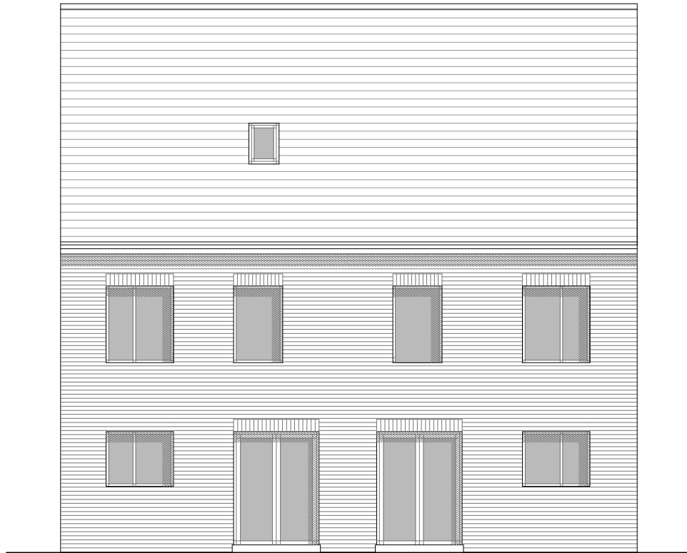
C - Rear Elevation
