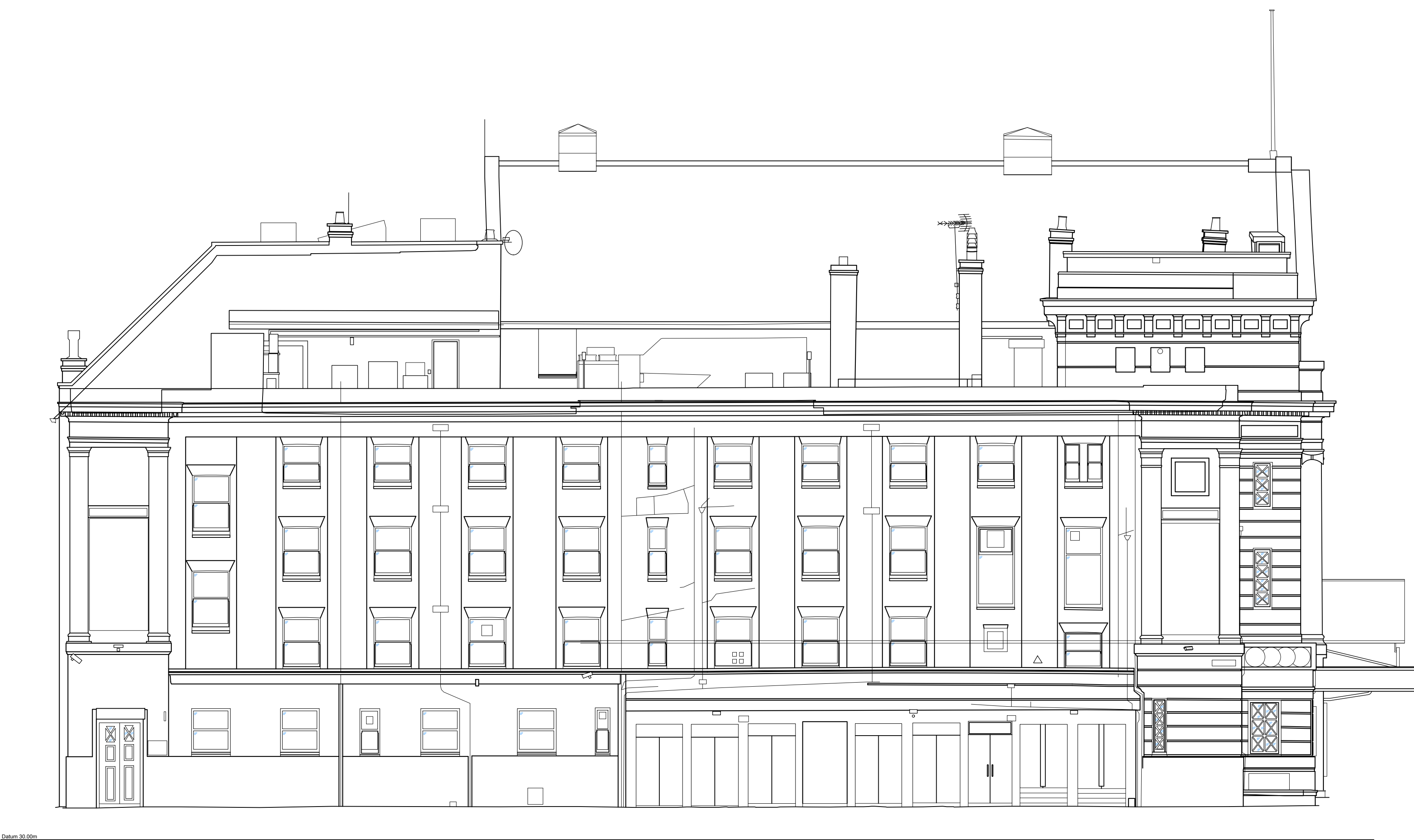
PROPOSED BYROM STREET ELEVATION 1:100
