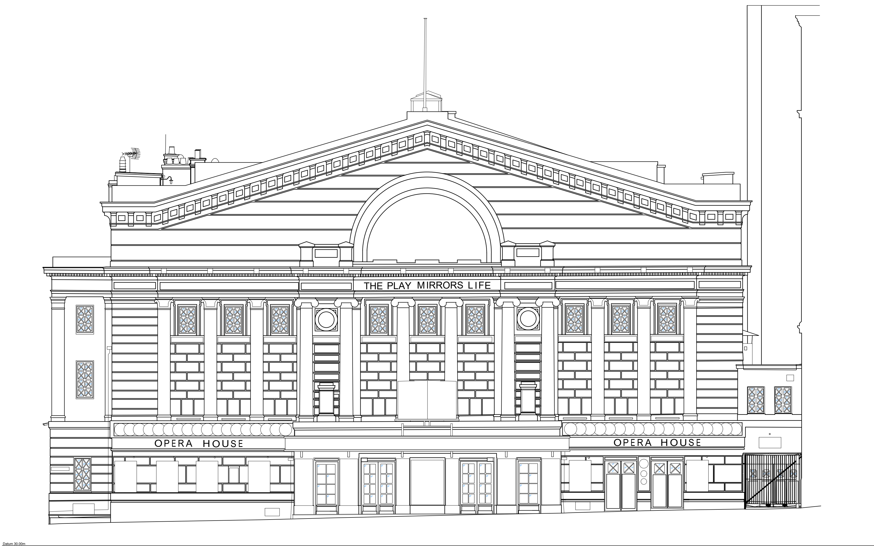
PROPOSED QUAY STREET ELEVATION 1:100
