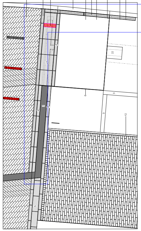
D1 Detail Plan of Outlet Interface Scale 1:25
