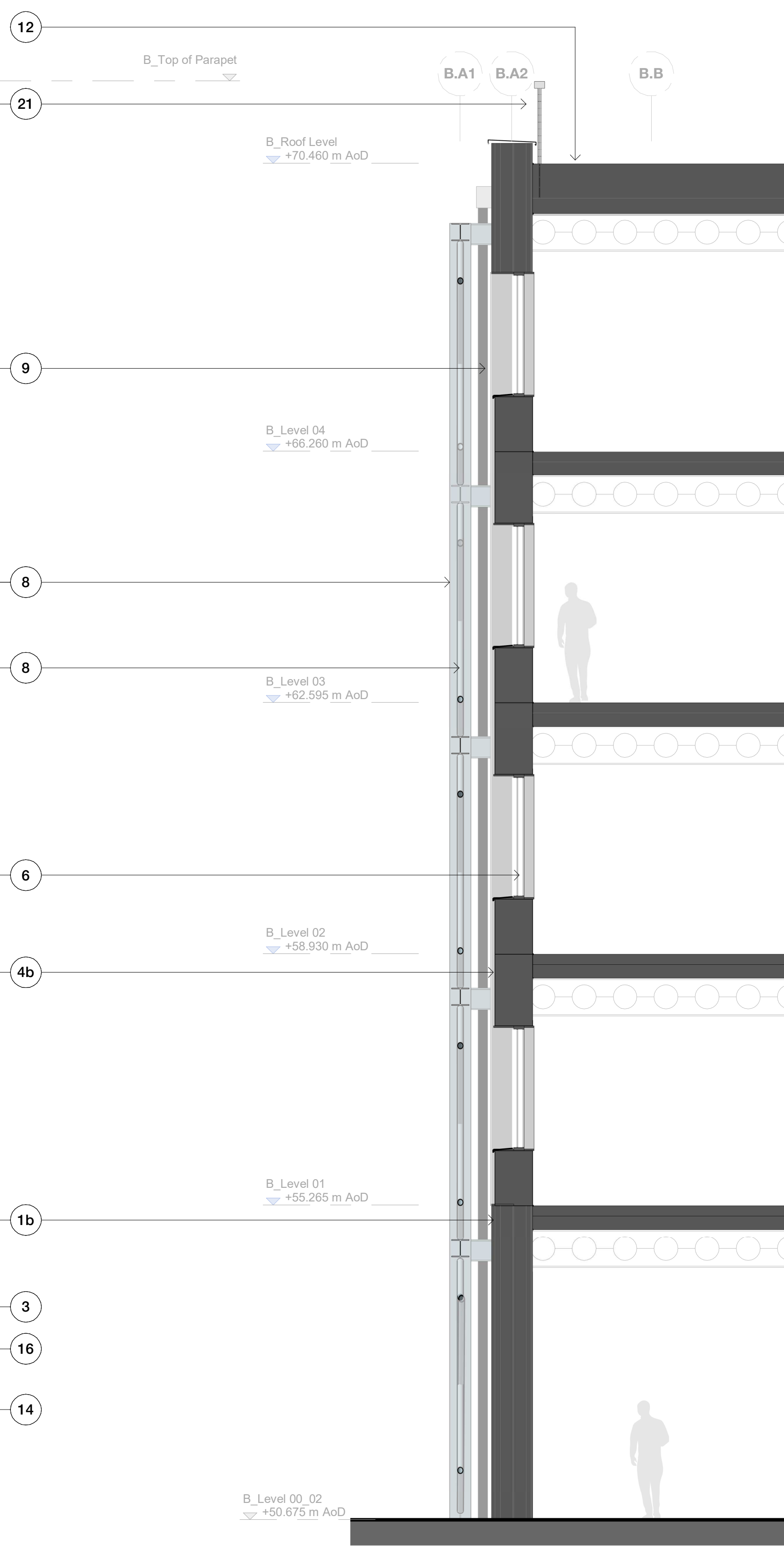
Building B - Section AA 1 : 50
