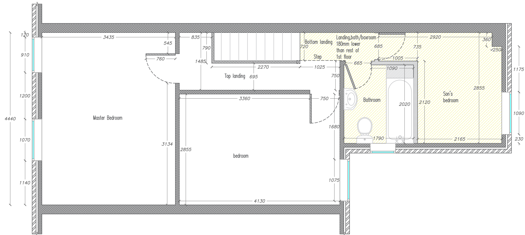
Existing 1st floor layout
