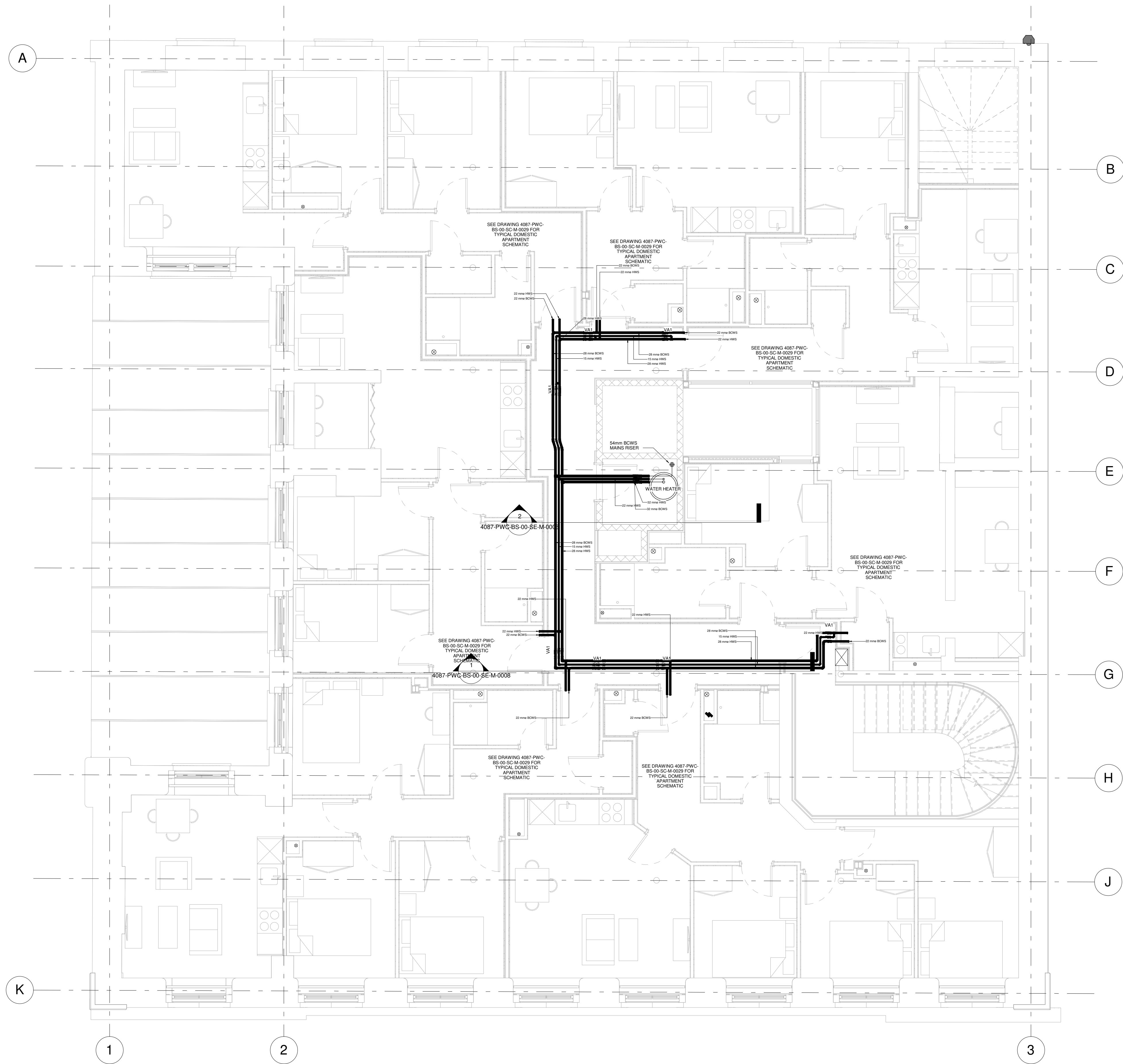
01 - Domestic Services Layout 1:50
