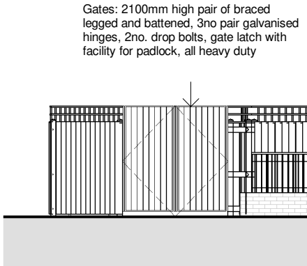
West Elevation (1:100)
