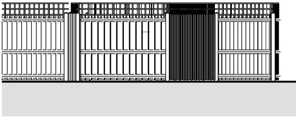
East Elevation (1:100)
