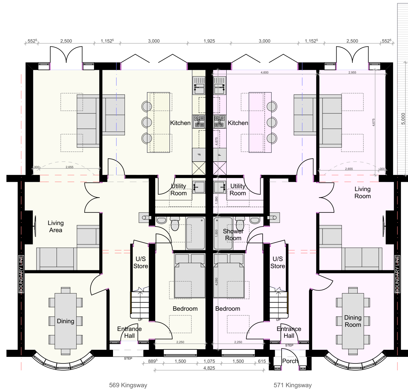
PROPOSED GA GROUND FLOOR PLANS
