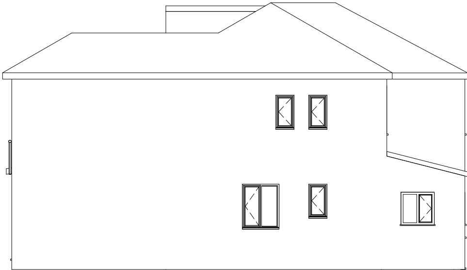
2 Side Elevation - Proposed 1 : 100
