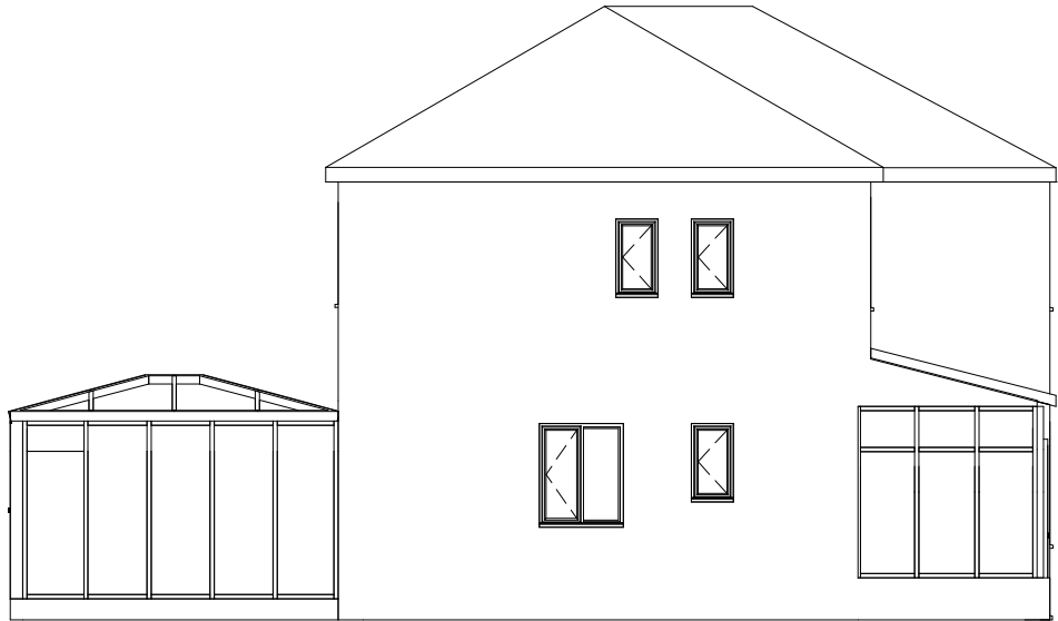
1 Side Elevation - Existing 1 : 100
