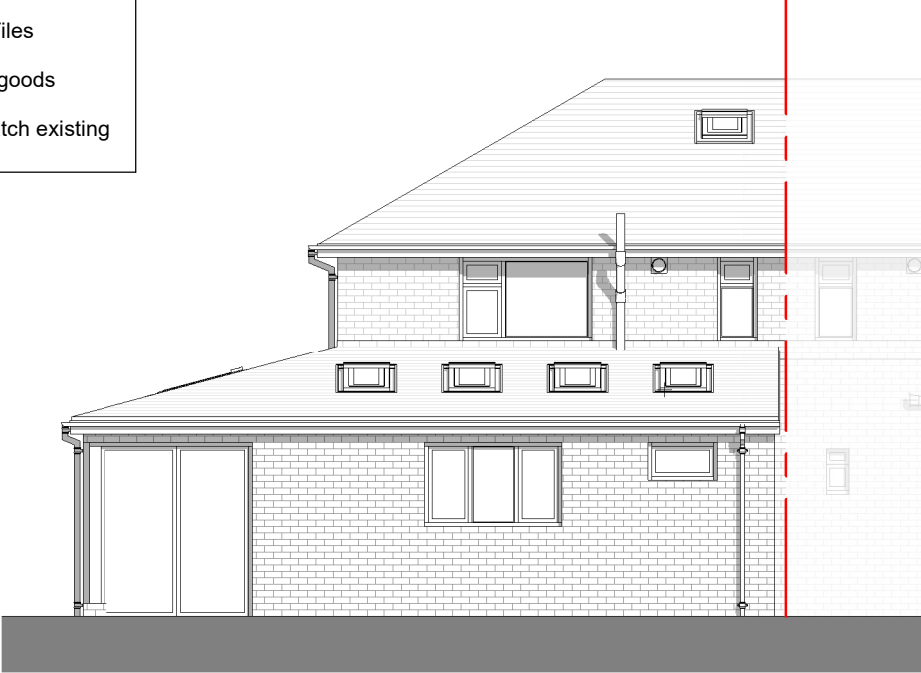
Rear Elevation 1 : 100
