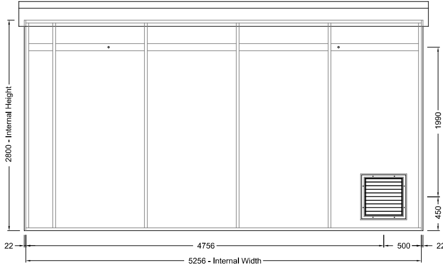
LH SIDE ELEVATION
