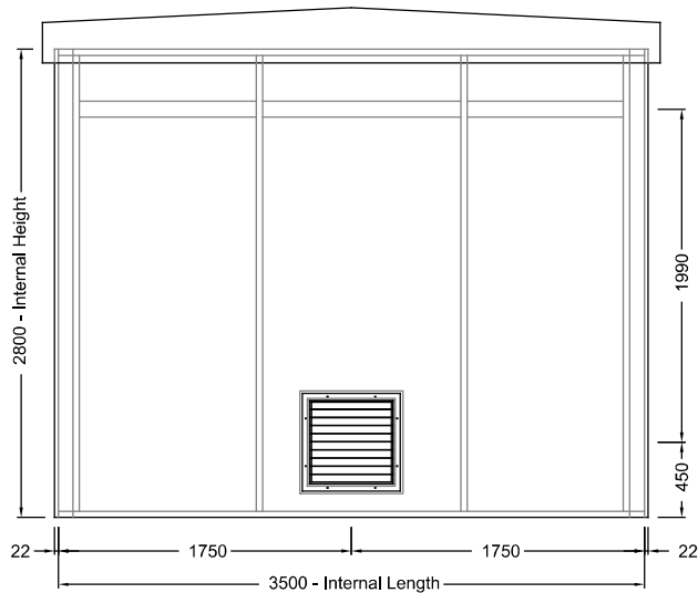
REAR ELEVATION
