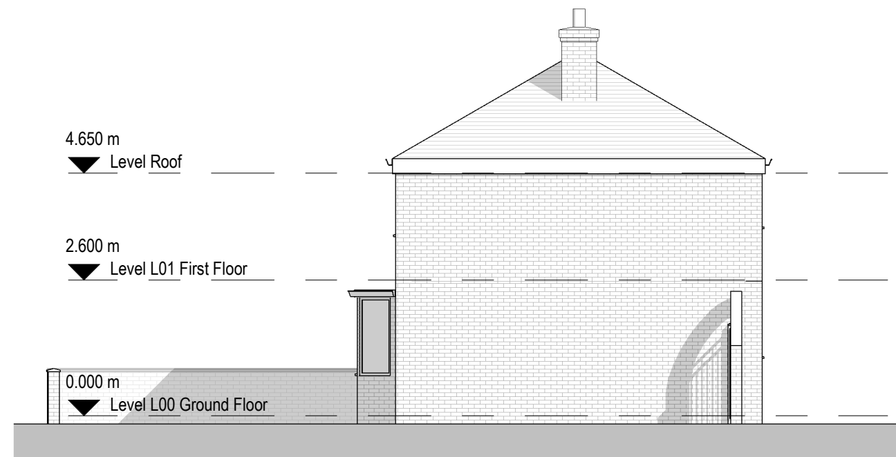
4 Existing East Elevation 1 : 100
