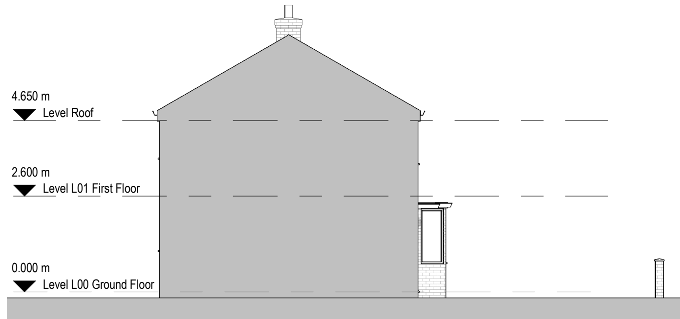
2 Existing West Elevation 1 : 100
