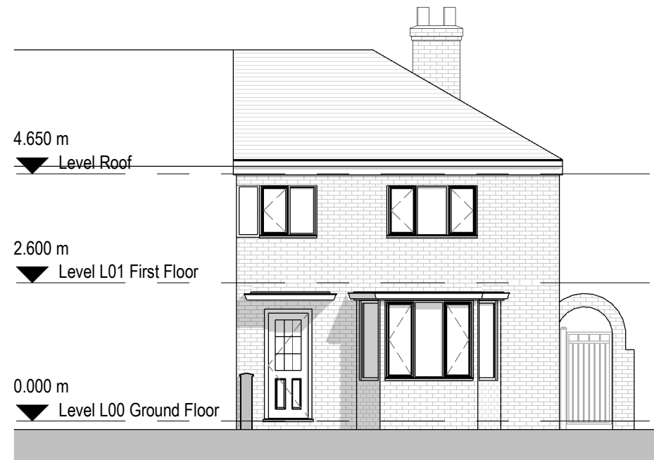
1 Existing South Elevation 1 : 100
