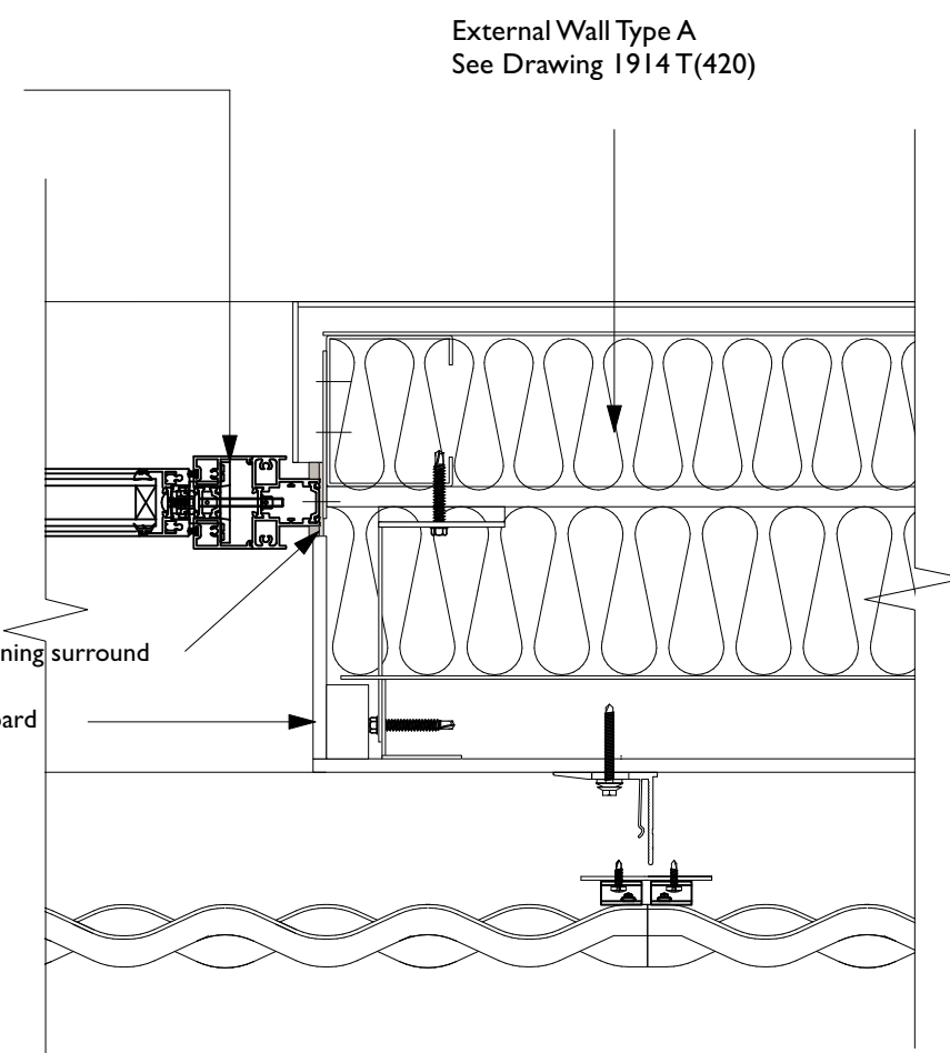
3 Glazed Slot Jamb Detail Scale: 1:5
