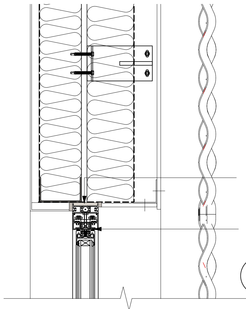
1 Glazed Slot Head Detail Scale: 1:5
