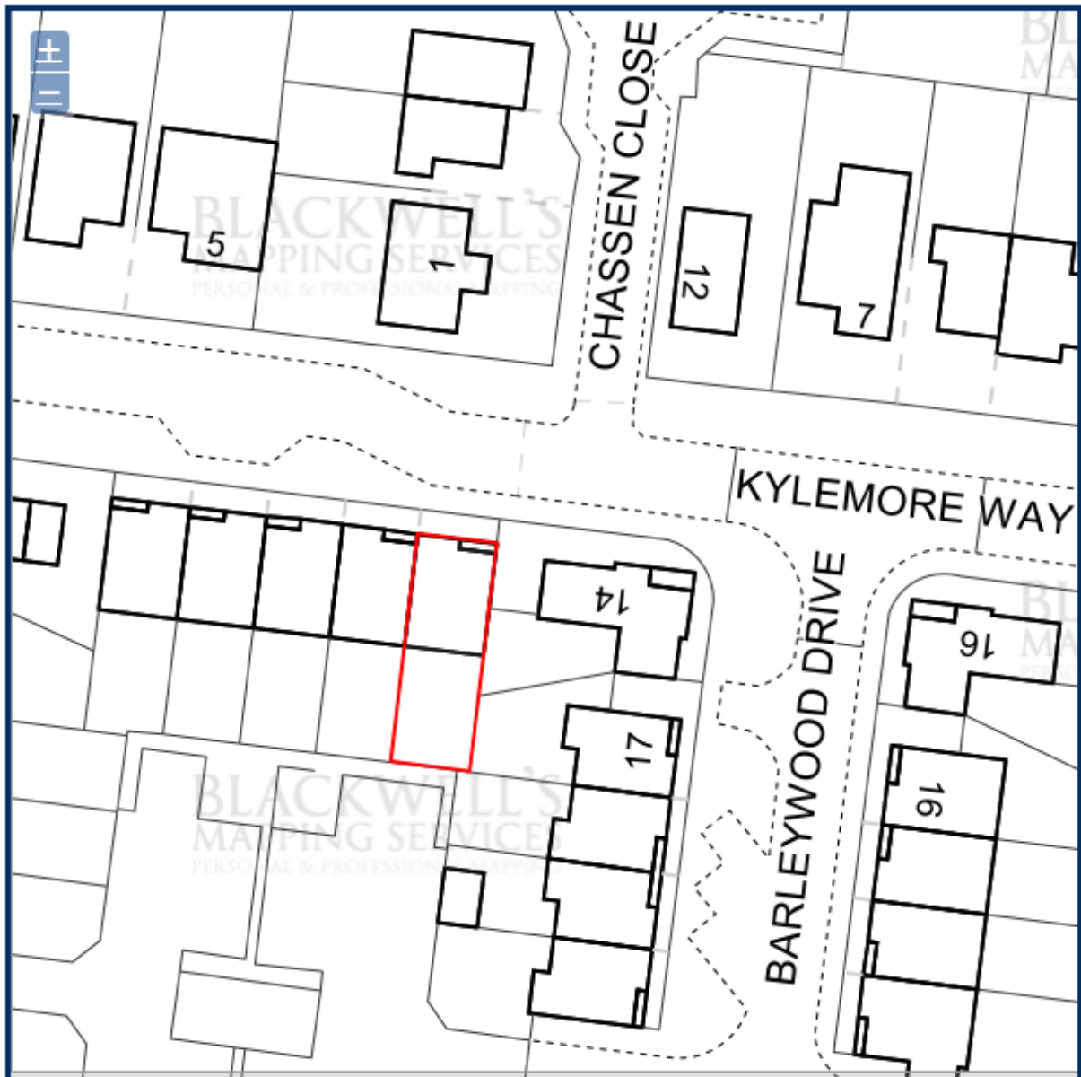
Existing block plan for 12 Kylemore Way, Manchester, M11 3LH - Scale @ 1:500 @ A3
