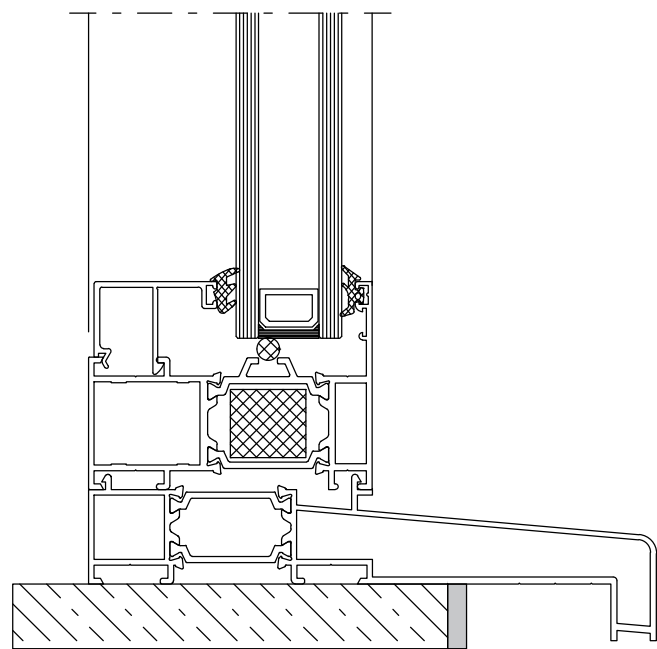
TYPICAL STATIC WINDOW (WITHIN BRICKWORK) VERTICAL SECTION SCALE 1:2 @A1
