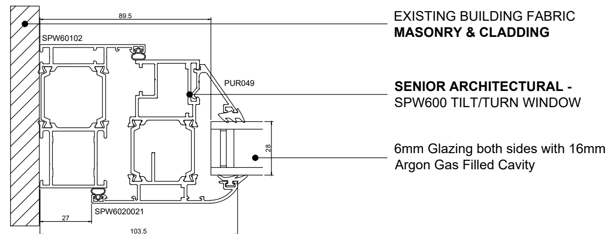
TYPICAL TILT/TURN WINDOW (WITHIN BRICKWORK) HORIZONTAL SECTION SCALE 1:2 @A1
