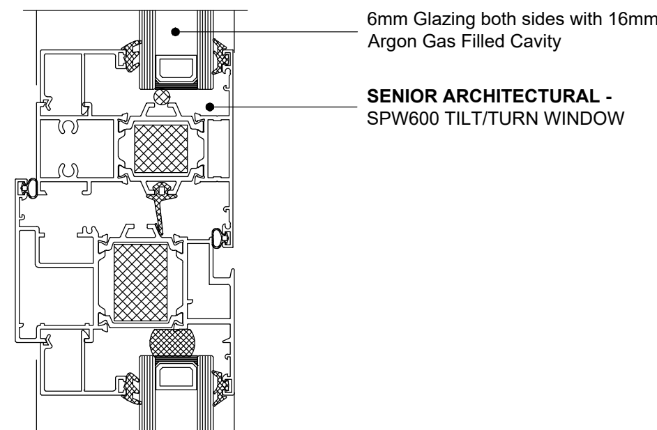
TYPICAL CURTAIN WINDOW VERTICAL SECTION SCALE 1:2 @A1
