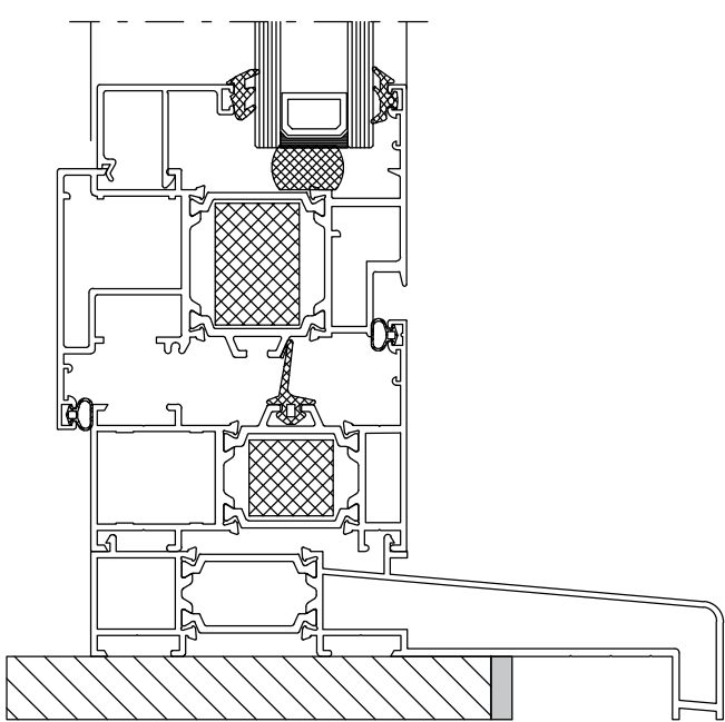
TYPICAL TILT/TURN WINDOW (WITHIN BRICKWORK) VERTICAL SECTION SCALE 1:2 @A1
