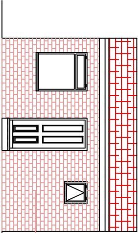
Proposed Extension Elevation
